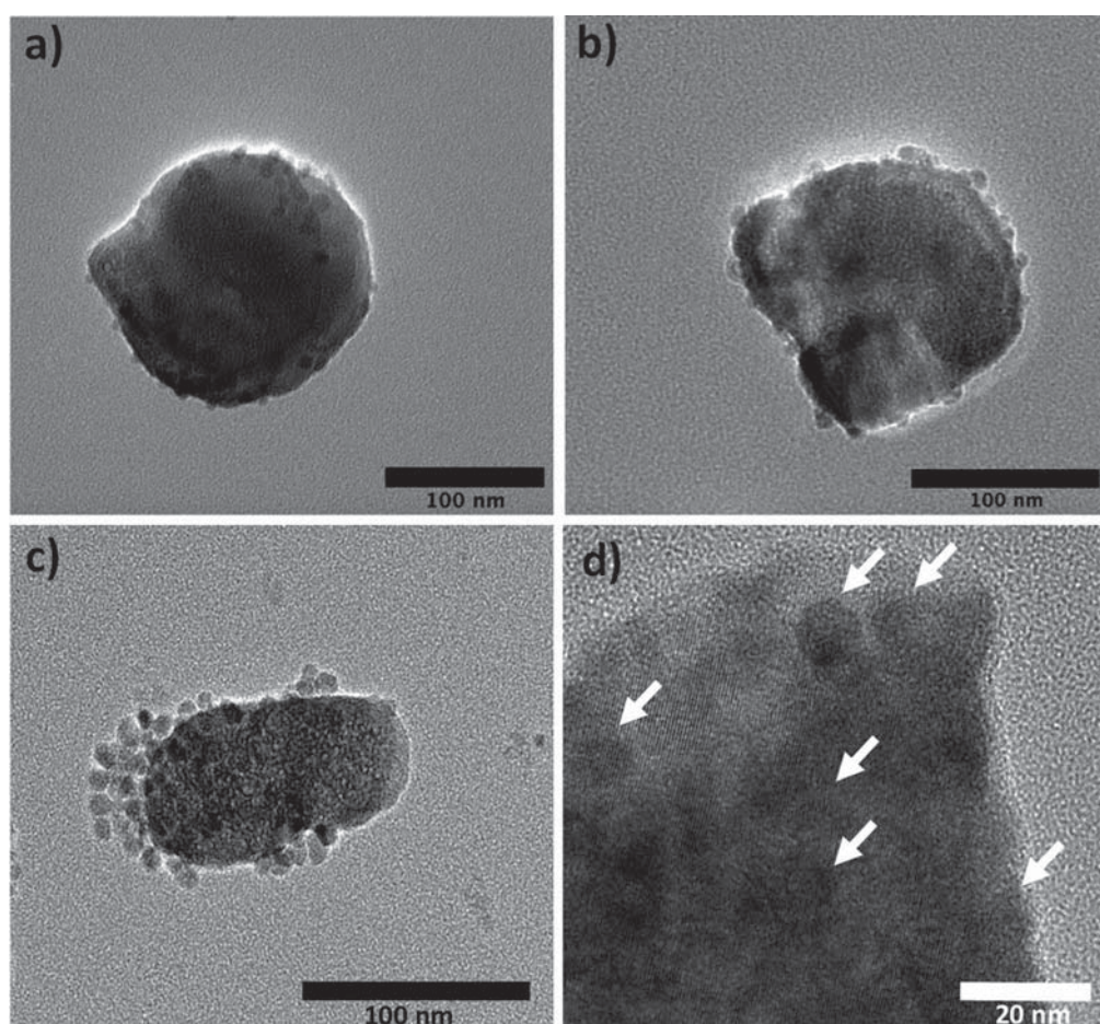
Fig. 5 (a–c) TEM micrographs of representative \beta - \text{NaY}_{0.8}[\text{Yb}_{0.18}\text{Er}_{0.02}]\text{F}_4@ \gamma - \text{Fe}_2\text{O}_3 core@satellite particles. (d) An HRTEM image of the border of a core@satellite particle is given to highlight (see white arrows) the attachment of the \gamma - \text{Fe}_2\text{O}_3 nanocrystals at the surface of the \beta - \text{NaY}_{0.8}[\text{Yb}_{0.18}\text{Er}_{0.02}]\text{F}_4 core. For these composite particles, a whole diameter ranging mainly between 110 and 160 nm was measured.
