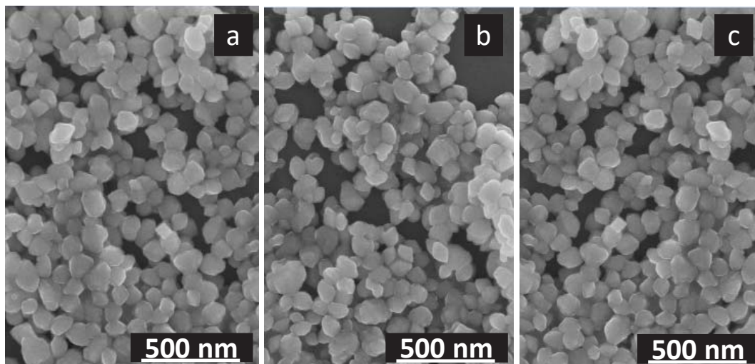
Figure S4. SEM Images recorded on the as-produced (a) \beta\text{-NaY}_{0.8}\text{[Er}_{0.2}\text{]F}_4 , (b) \beta\text{-NaY}_{0.8}\text{[Yb}_{0.2}\text{]F}_4 and (c) \beta\text{-NaY}_{0.8}\text{[Yb}_{0.18}\text{Er}_{0.02}\text{]F}_4 powders.
