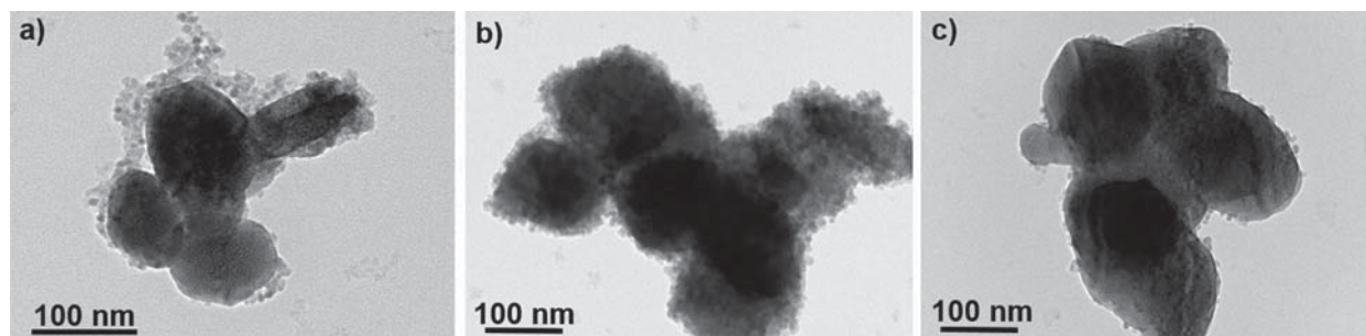
Fig. 4 TEM micrograph of an assembly of (a) \beta - \text{NaY}_{0.8}[\text{Er}_{0.2}]\text{F}_4@ \gamma - \text{Fe}_2\text{O}_3 , (b) \beta - \text{NaY}_{0.8}[\text{Yb}_{0.2}]\text{F}_4@ \gamma - \text{Fe}_2\text{O}_3 and (c) \beta - \text{NaY}_{0.8}[\text{Yb}_{0.18}\text{Er}_{0.02}]\text{F}_4@ \gamma - \text{Fe}_2\text{O}_3 particles.
