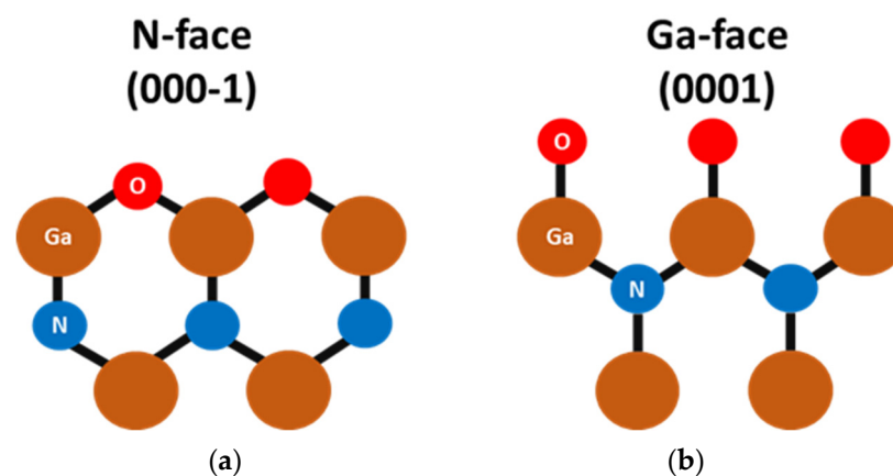
Figure 1. Side view diagram of the N-face (a) and Ga-face (b) GaN in the presence of oxygen atoms.
