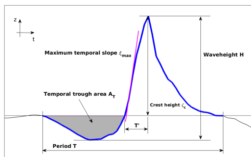
FIG. 2. Definition sketch of wave parameters used here. Waveheight H , crest height \zeta_c , wave period T , wave front period T' , temporal trough area A_T (units: meters-seconds) and maximum temporal slope \xi_{max} (units: meters / seconds).
