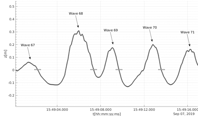
FIG. 3. Segmentation of the wave record. A zero down-crossing segmentation is applied to each wave record. In this figure, five waves in the record Cv48 at Pole 2 are shown (Wave 67 through Wave 71). The white bar designates the demarcation of two different wave events. For each wave in each record the basic parameters indicated in Figure 2 are found, and the six quantities delineated in Table 1 are computed.
