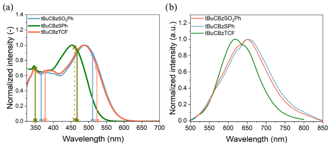
Figure 2. Experimental absorption (a) and emission (b) spectra of investigated compounds in THF solution C \sim 1.5 \times 10^{-5} \text{ mol/dm}^3 . The emission spectra were recorded at room temperature using an excitation wavelength equal to the maximum absorption for each compound. Vertical lines indicate maxima computed for S_0 \rightarrow S_1 and S_0 \rightarrow S_3 transitions calculated by the TD-DFT approach (the details can be found in the Experimental Section). The continuous lines with dots at the ends represent more stable conformers, while dashed lines with crosses at the ends are less stable conformers. Inset in part a shows the molecular structure of investigated compounds.
