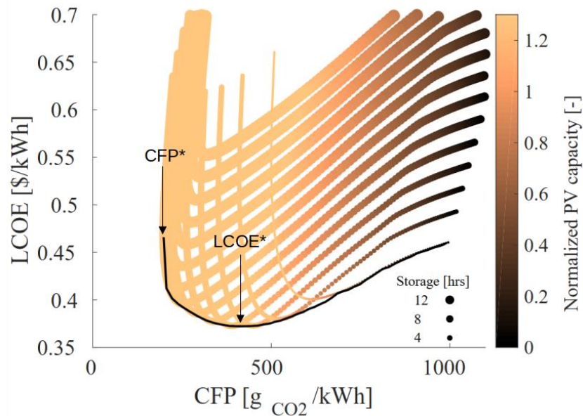
2 3 4 5 6 7 8 9 Figure 3: Lowest LCOE ( LCOE^* ) and lowest CFP ( CFP^* ) configurations in a LCOE vs. CFP graph. The black line is the envelope curve. The colour shows the normalized PV capacity installed (dark dots refer to configurations with low penetration of solar, and light dots to high penetration of solar) while the size of the dots reflects the normalized storage capacity installed. Each U-shape line depicts a given storage capacity (only one out of three storage capacities simulated is represented). Each dot of each line corresponds to a given PV capacity. Each dot reflects a given genset production, i.e., the production required to satisfy the demand throughout the period. The storage capacity, the PV capacity and the genset production allow to estimate the CFP and the LCOE of the configuration. This graph is obtained for a location in Angola ( -12.5^{\circ}N ; 17.5^{\circ}E ) with a hybrid load profile.
