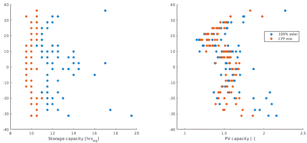
6 7 8 9 10 Figure B.3 : Configurations (PV and storage capacities) for the CFP* configurations (red) and configurations which supply more than 99% of the energy with solar PV (blue). This figure shows only the result for a hybrid load profile without seasonality. Imposing a strong constraint (>99%) on the proportion of energy covered by solar PV increases the storage capacity, whereas the PV capacity stays similar.
