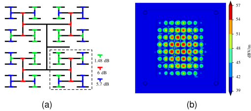
Fig. 4. (a) Weight ratios in the splitters and (b) E-field amplitude at 30 GHz.
