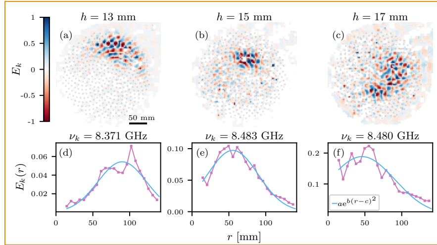
Fig. 9. [(a), (b), and (c)] Spatial modal structure and [(d), (e), and (f)] the radial profile of representative Gaussian eigenmodes. Quality factor of the modes: (a) Q_k \approx 3931 ; (b) Q_k \approx 4375 ; (c) Q_k \approx 3586 . Amplitude maps are normalized such that \max(|E_k|) = 1 . Radial decays (pink dots) are obtained by performing an angle averaging where r = \sqrt{(x+5)^2 + y^2} is measured from the center of the spiral and expressed in mm.
