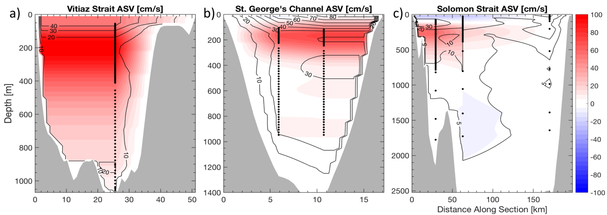
Figure 4. The mean (red-blue color map) and standard deviation (black contours) of the along-strait velocity (ASV; cm/s) for (a) Vitiaz Strait, (b) St. George's Channel, and (c) Solomon Strait. Statistics were calculated over the deployment period, and the vertical limits are the ocean surface to each channel's respective sill depth. Mean ASV sections are contoured at 5 cm/s increments, and red indicates transport exiting the Solomon Sea, while blue indicates transport entering. The standard deviation of the ASV is contoured in 10 cm/s intervals with an additional 5 cm/s contour for Solomon Strait. Deployment-mean locations of all ADCP bins and single point current meters are indicated with black dots for the directly observed velocity sections. Due to close vertical spacing of some ADCP bins, black dots may appear as thick vertical lines. Note the discontinuity across Solomon Strait is due to the discontinuous transect line used for the channel cross section (Figure 1b).
