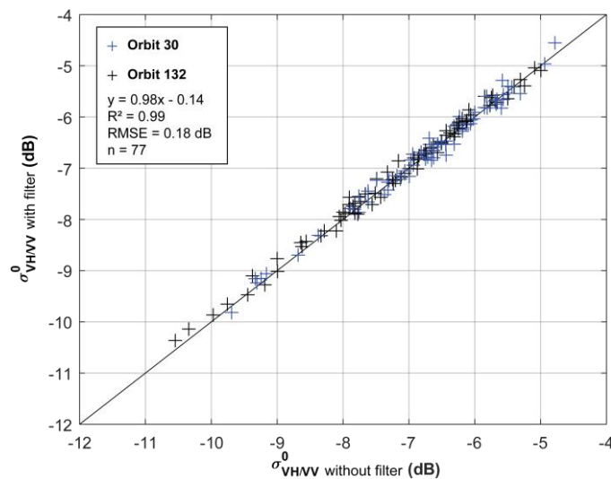
Figure 12. Comparison of the backscattering coefficient ( \sigma^{\circ}_{VH/VV} ) extracted at a field scale (between 0 and 1000 °C day), with or without considering a 3 \times 3 window adaptive Lee filter. Black and blue crosses represent the backscattering coefficients acquired in orbit 132 and 30, respectively.
