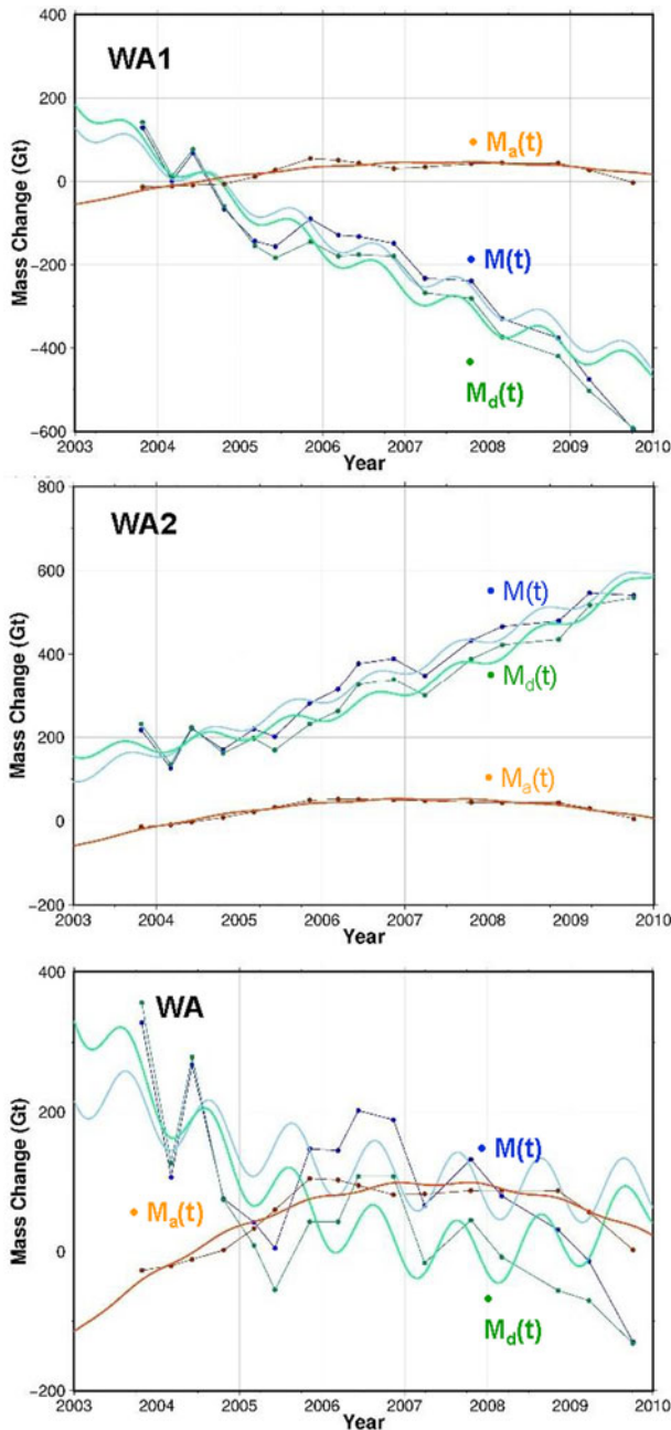
Fig. 8. Components of mass change from ICESat for WA, WA1 and WA2 from M_d(t) = \rho_{ice} \times H_d(t) from Figure 7 and M_a(t) = \int^t \delta A(t) \times dt with LQS fit through 2008 data only. Linear trends and the adjusted dB_{cor} and GIA_{cor} applied are in Table 3. The dynamic M_d(t) is more linear than the total M(t) .
