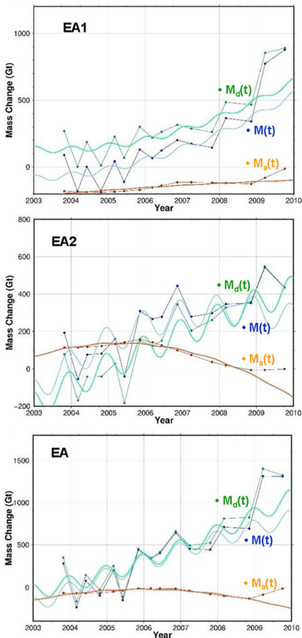
Fig. 6. Components of mass change from ICESat for EA, EA1 and EA2 from M_d(t) = \rho_{\text{ice}} \times H_d(t) from Figure 5 and M_a(t) = \int^t \delta A(t) \times dt with LQS fit through 2008 data only. Linear trends and the adjusted \delta B_{\text{cor}} applied are in Table 3. The dynamic M_d(t) is more linear than the total M(t) .
