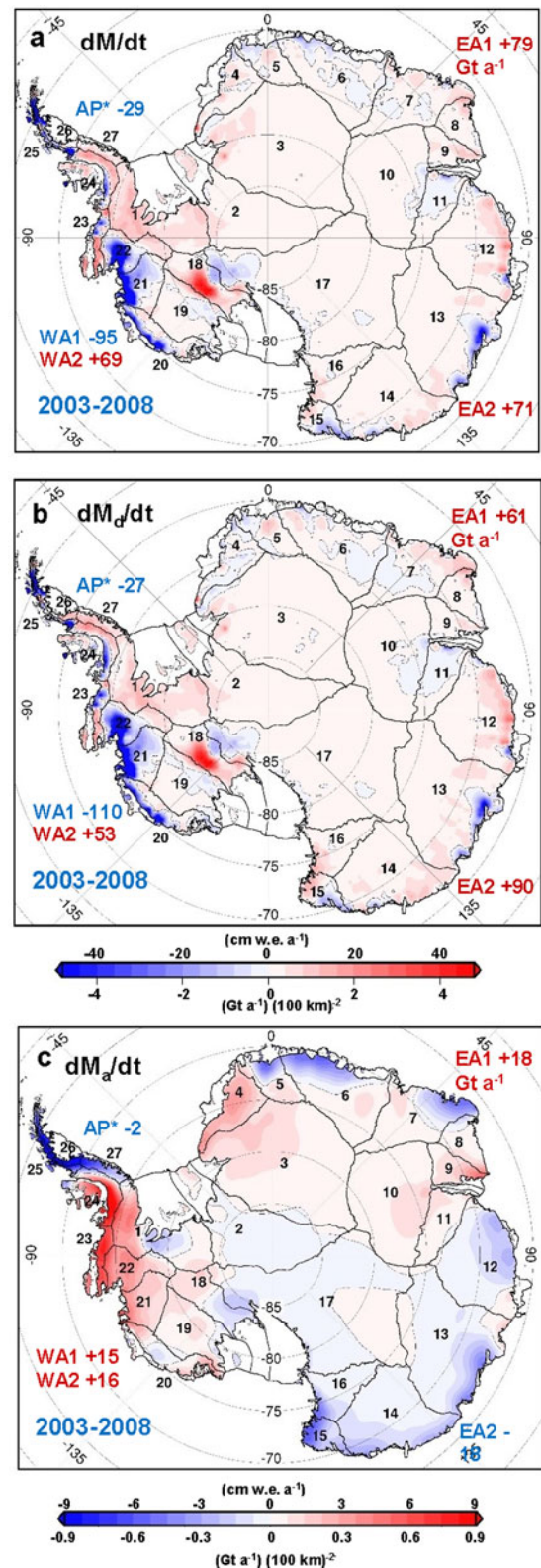
Fig. 16. ICESat maps for 2003–2008, (a) dM/dt , (b) dM_d/dt and (c) dM_a/dt using \delta B/dt equal to \text{Ivins}\delta B/dt + \delta B_{\text{adj}} . Rates are linear terms of LQS fits at year 2006.0. *Rates for AP from average-linear-change analysis.
