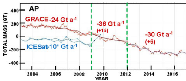
Fig. 14. M(t) time-series for Antarctic Peninsula from ICESat (blue) and GRACE (red) using dB_{\text{cor}} = -0.5 \text{ a}^{-1} and GIA_{\text{cor}} = -2.3 \text{ Gt a}^{-1} from Ivins2. The linear trends from LQS fits at the midpoints of 2003–2009, 2009–2012 and 2012–2016.3 are also in Table 7a. *The -10 \text{ Gt a}^{-1} from LQS is replaced by -29 \text{ Gt a}^{-1} from average-linear change analysis in AIS sum in Figure 15 and Table 7a.
