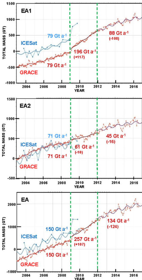
Fig. 12. M(t) time series for East Antarctica from ICESat (blue) and GRACE (red) using the equalizing dB_{cor} and GIA_{cor} listed in Table 3. The linear trends from LQS fits at the midpoints of 2003–2009, 2009–2012 and 2012–2016.3 also in Table 7a.
