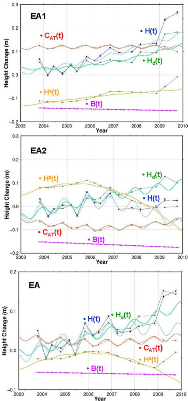
Fig. 5. Components of elevation change from ICESat for EA, EA1 and EA2 from H_d(t) = H(t) - H^a(t) - C_{AT}(t) - (dB/dt) \times t with LQS fit through 2008 data only. Linear trends and the adjusted dB/dt used for B(t) are in Table 3. The dynamic H_d(t) is more linear than other elevation terms.
