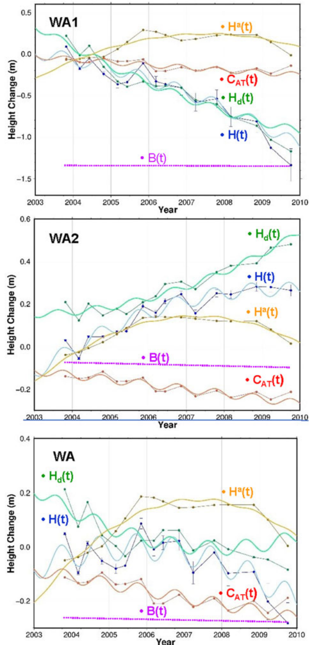
Fig. 7. Components of elevation change from ICESat for WA, WA1 and WA2 from H_d(t) = H(t) - H^a(t) - C_{AT}(t) - (dB/dt) \times t with LQS fit through 2008 data only. Linear trends and the adjusted dB/dt used for B(t) are in Table 3. The dynamic H_d(t) is more linear than H(t) and other elevation terms.
