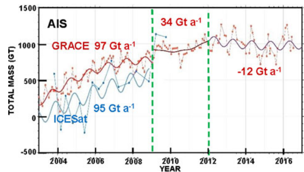
Fig. 15. M(t) time series for Antarctica from ICESat (blue) and GRACE (red). The linear trends from LQS fits at the midpoints of 2003–2009, 2009–2012 and 2012–2016.3 are also in Table 7a.
