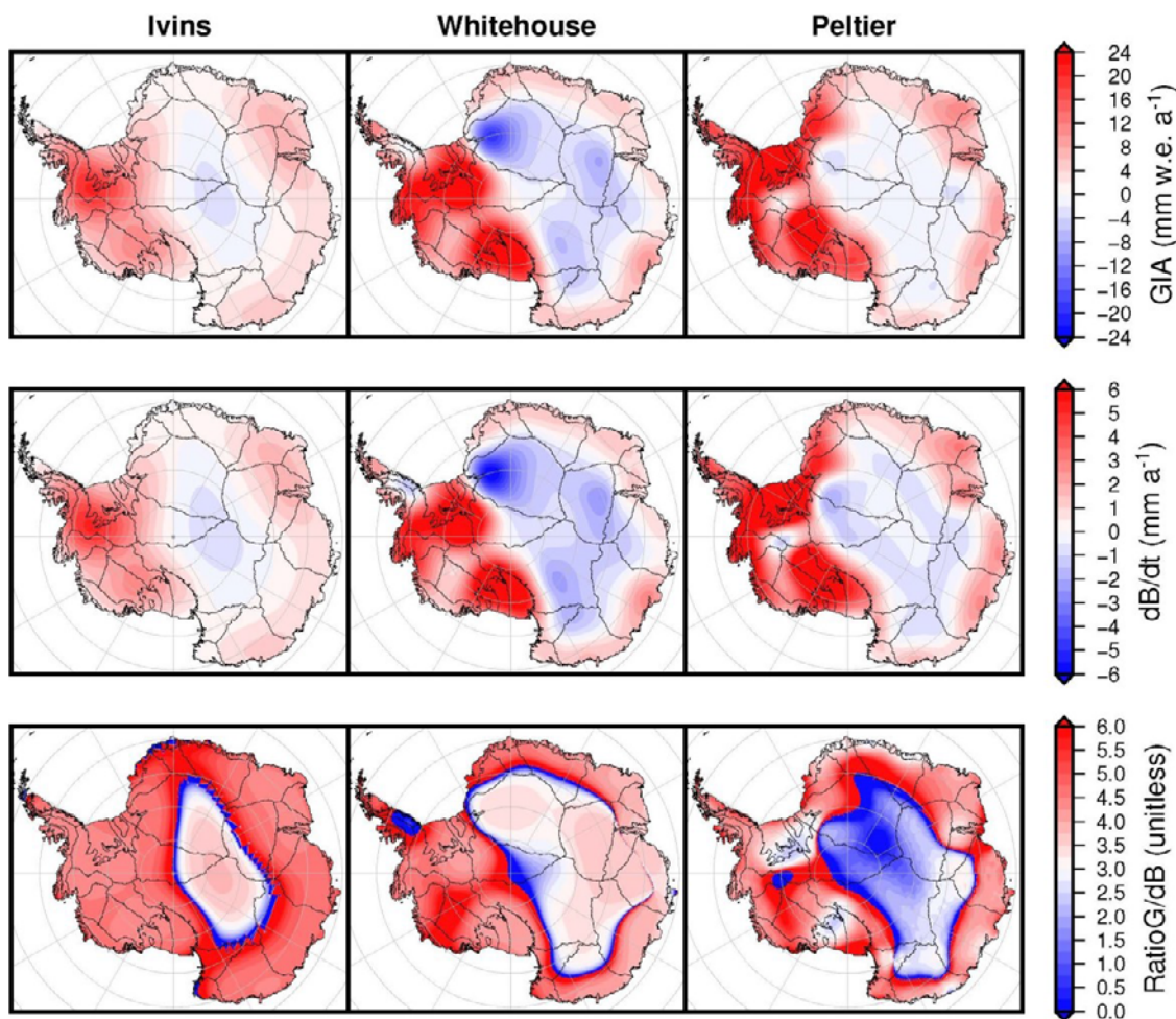
Fig. 3. Glacial Isostatic Adjustment (GIA) in mm w.e. a -1 , basal uplift (dB/dt) in mm a -1 , and RatioG/dB equal to GIA/(0.91 \times dB/dt) derived by three Earth models labeled Ivins, Whitehouse and Peltier (Whitehouse and others, 2012; Ivins and others, 2013; Peltier, 2014). Subsidence rate from glacial loading in the central part of EA ice sheet is largest in Whitehouse model and smallest in Ivins.
