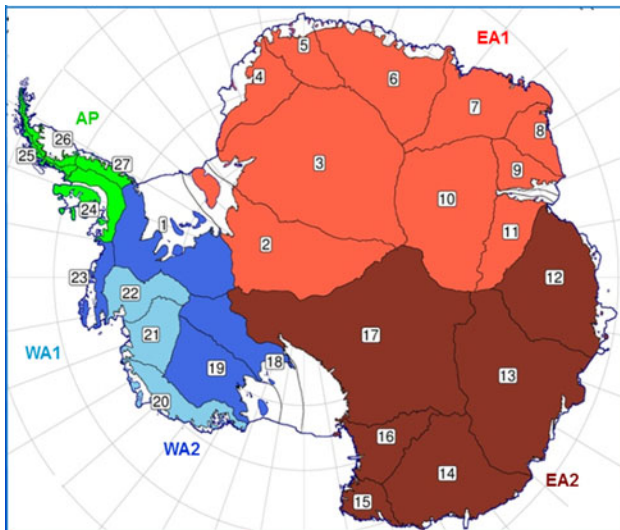
Fig. 1. Antarctic ice sheet regions and drainage systems. East Antarctica (EA) is divided into EA1 (DS2 to DS11) and EA2 (DS12 to DS17). The Antarctic Peninsula (AP) includes DS24–27. West Antarctica (WA) is divided into WA1 (Pine Island Glacier DS22, Thwaites and Smith Glaciers DS21, and the coastal DS20) and WA2 (inland DS1, DS18, and DS19 and coastal DS23). Includes grounded ice within ice shelves and contiguous islands.
