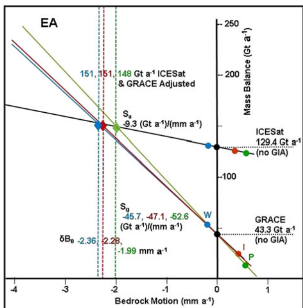
Fig. 11. ICESat and GRACE dM/dt for EA with no \delta B_{cor} or GIA_{cor} corrections (●) and with corrections from models of Ivins (●), Peltier (●) and Whitehouse (●). ICESat and GRACE equalized dM/dt mass changes range from 148 Gt a^{-1} using S_g = -52.6 Gt a^{-1}/mm a^{-1} and \delta B_0 = -1.99 mm a^{-1} from Peltier model, to 151 Gt a^{-1} using S_g = -47.1 Gt a^{-1}/mm a^{-1} and \delta B_0 = -2.28 mm a^{-1} from Ivins model, to 151 Gt a^{-1} using S_g = -45.7 Gt a^{-1}/mm a^{-1} and \delta B_0 = -2.36 mm a^{-1} from Whitehouse model.
