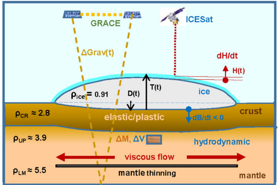
Fig. 2. Ice sheet of thickness, T , lying on Earth’s crust and underlying fluid mantle. For long-term isostatic equilibrium ( \sim 10 ka) with constant ice thickness the depth of the depression would be D \approx \rho_{ice} / \rho_{mantle} \times T , which is 600 m for T = 3000 m and \rho_{mantle} = 4.5 , and the dB/dt would be zero. As the glacial loading, T(t) , on the Earth’s crust continually changes, the underlying viscous mantle hydrodynamically adjusts over centuries to millennia. Illustration is for an increasing ice thickness that induces a downward motion of the crust (i.e. dB/dt < 0 ), outward mantle flow and mantle thinning. For this case, the GRACE senses the gravitational changes of the increasing ice mass minus the decreasing mantle mass ( \Delta M ) under the satellite. ICESat senses the increase in ice thickness minus the downward motion of the crust and mantle caused by the change in mantle volume ( \Delta V ).
