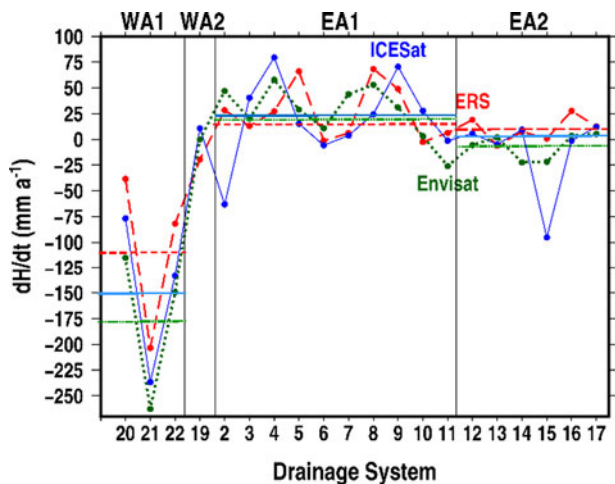
Fig. 10. Average dH/dt from ERS1/2 1992–2001 (dashed red), ICESat 2003–2008 (solid blue) and Envisat 2002.7–20010.7 (dotted green) by DS and sub-regions for areas of common coverage. DS20, 21, 22, 19 and 4 to 16 are completely covered.
