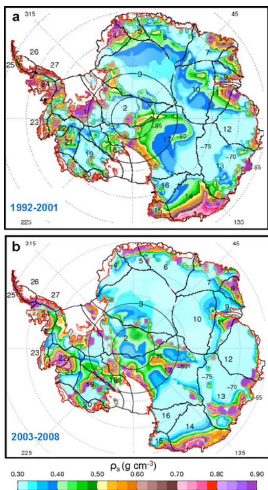
Fig. 17. Maps of the calculated firn density \rho_a = \Delta M_a / \Delta(H^a - C_a) (see text following Eqn (16)) associated with the accumulation driven dM_a/dt mass changes for (a) 1992–2001 and (b) 2003–08, showing the large spatial and temporal variations.
