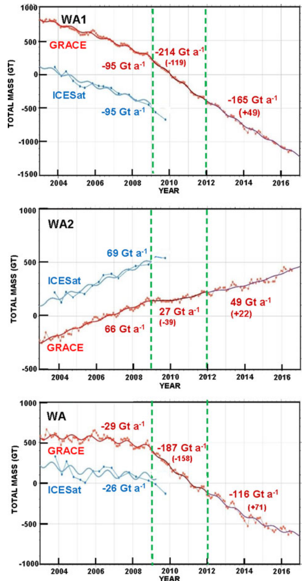
Fig. 13. M(t) time series for West Antarctica from ICESat (blue) and GRACE (red) using the equalizing dB_{cor} and GIA_{cor} listed in Table 3. The linear trends from LQS fits at the midpoints of 2003–2009, 2009–2012 and 2012–2016.3 also in Table 7a.
