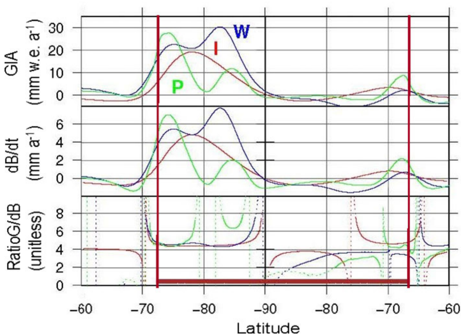
Fig. 4. Profiles of GIA, dB/dt and RatioG/dB from three dynamic Earth models Ivins (red), Peltier (green) and Whitehouse (blue) along 90°W across West Antarctica and along 90°E across East Antarctica extending into oceans. Singularities in RatioG/dB are avoided by calculating regional averages. Extent of continental ice is indicated by red lines.
