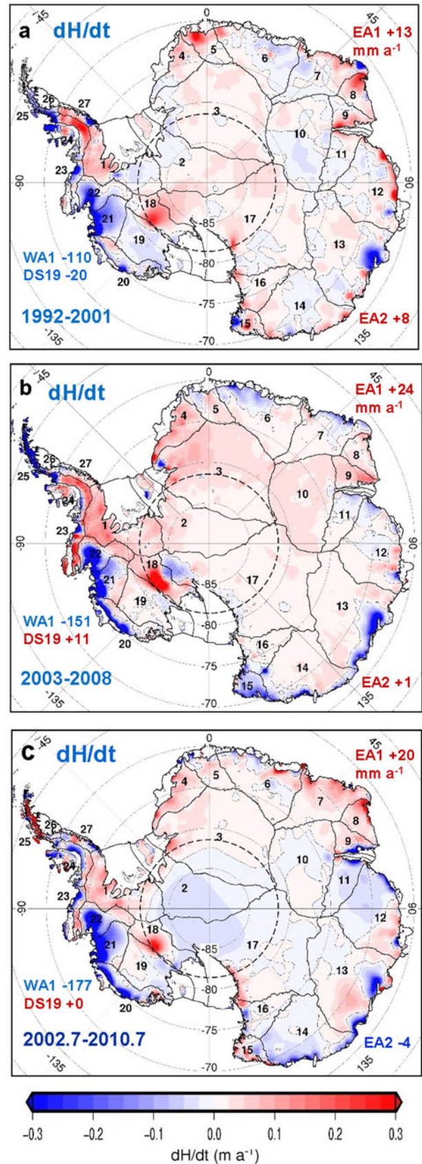
Fig. 9. Maps of dH/dt : (a) for 1992–2001 from ERS1/2, (b) for 2003–2008 from ICESat, and (c) for 2002.7–2010.7 from Envisat showing regional dH/dt for areas of common coverage. (Areas south of 81.6° coverage of ERS and Envisat and south of 86° of ICESat are interpolated in images.)
