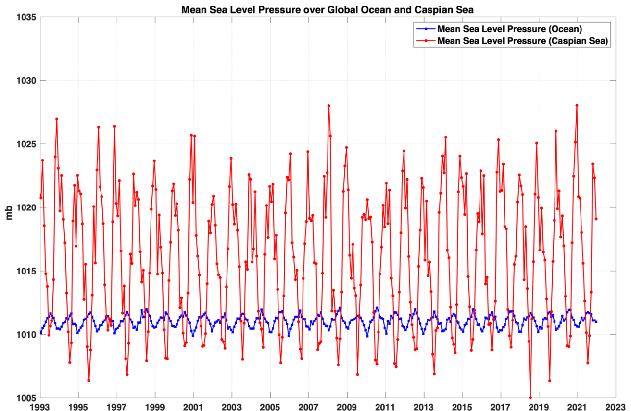
Figure 4. Monthly mean sea level pressure (in units of mb) over the global ocean (blue curve) and Caspian Sea (red curve) over the period January 1993 to December 2021, estimated from the ECMWF ERA5 mean sea level pressure data.
