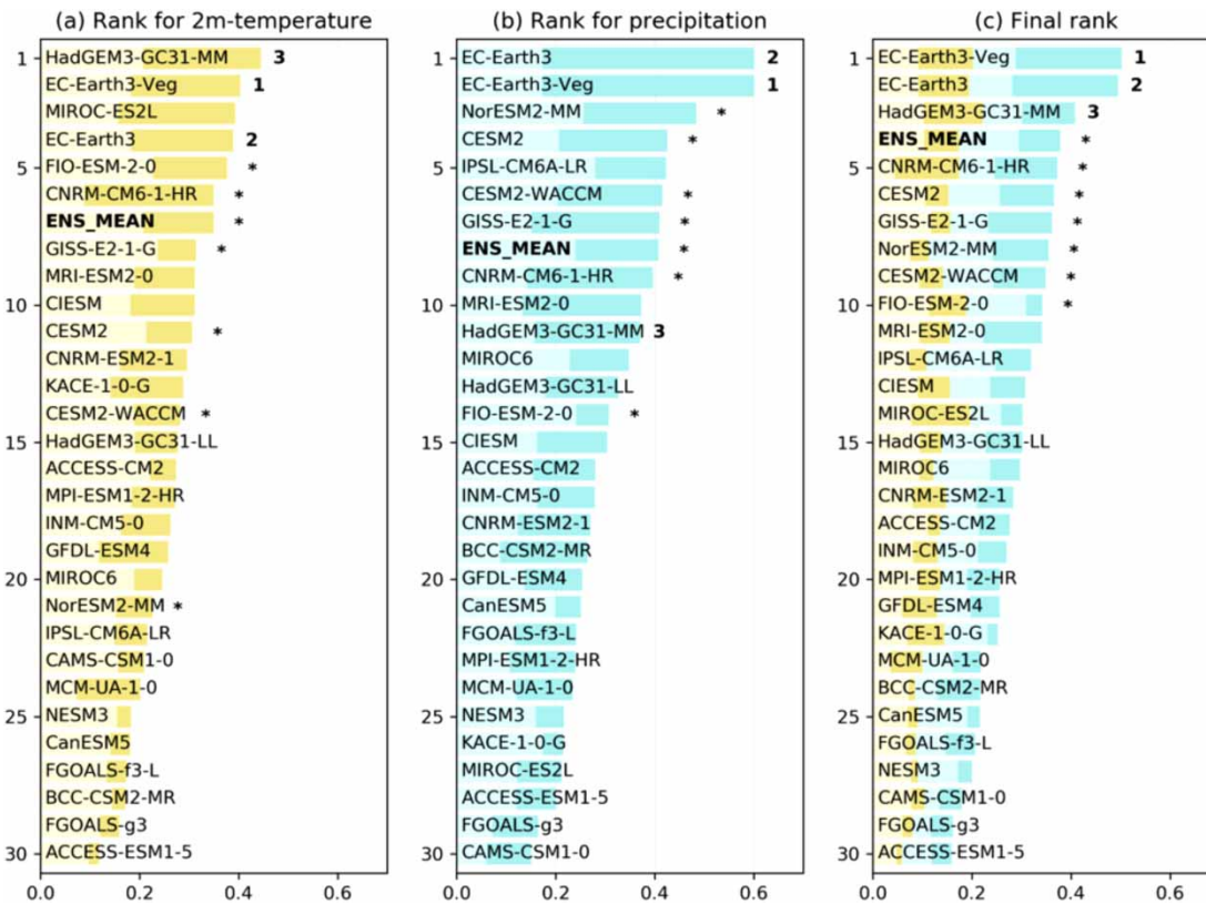
Figure 8 | Scores and ranks of 29 CMIP6 GCMs and their ensemble mean for (a) 2m-temperature (b) precipitation, and (c) all. Light and dark yellow highlight the contribution of temporal and spatial scores for temperature, respectively, while two shades of cyan are used similarly for precipitation. The top three models for Vietnam are labeled with numbers and the next seven models are marked with an asterisk. Please refer to the online version of this paper to see this figure in colour: https://dx.doi.org/10.2166/wcc.2023.454 .
