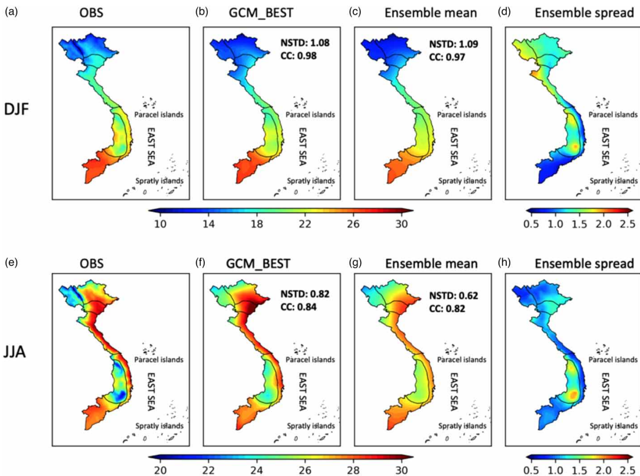
Figure 6 | Spatial distribution of DJF (upper panel) and JJA (lower panel) temperatures for (a,e) OBS, (b,f) the GCM that best represents temperature, (c,g) the ensemble mean, and (d,h) the standard deviation of all 29 models. Units in °C.
