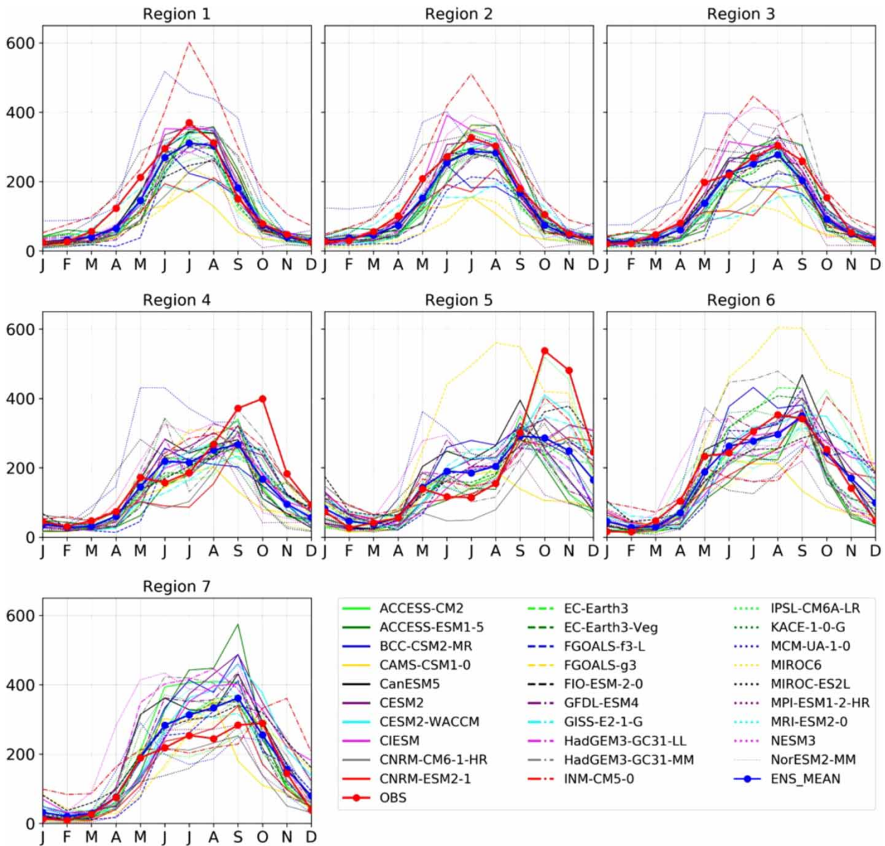
Figure 4 | Same as Figure 2 but for rainfall.
