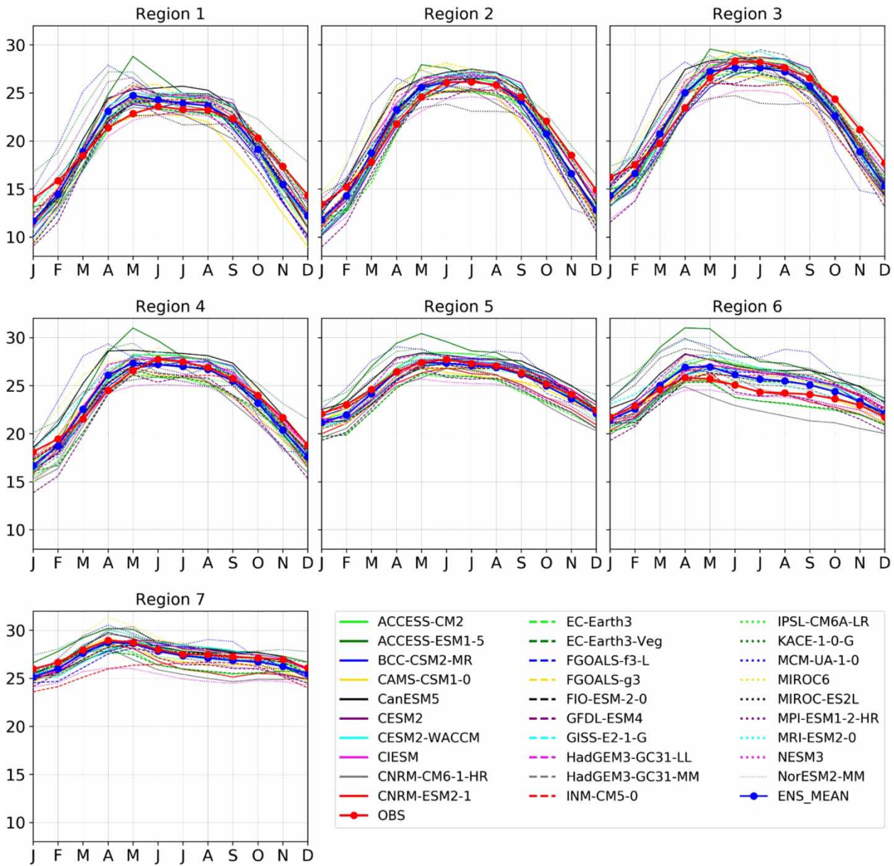
Figure 2 | Annual cycles of temperature over the seven sub-regions of Vietnam, represented by the GCMs and the reference dataset OBS.
