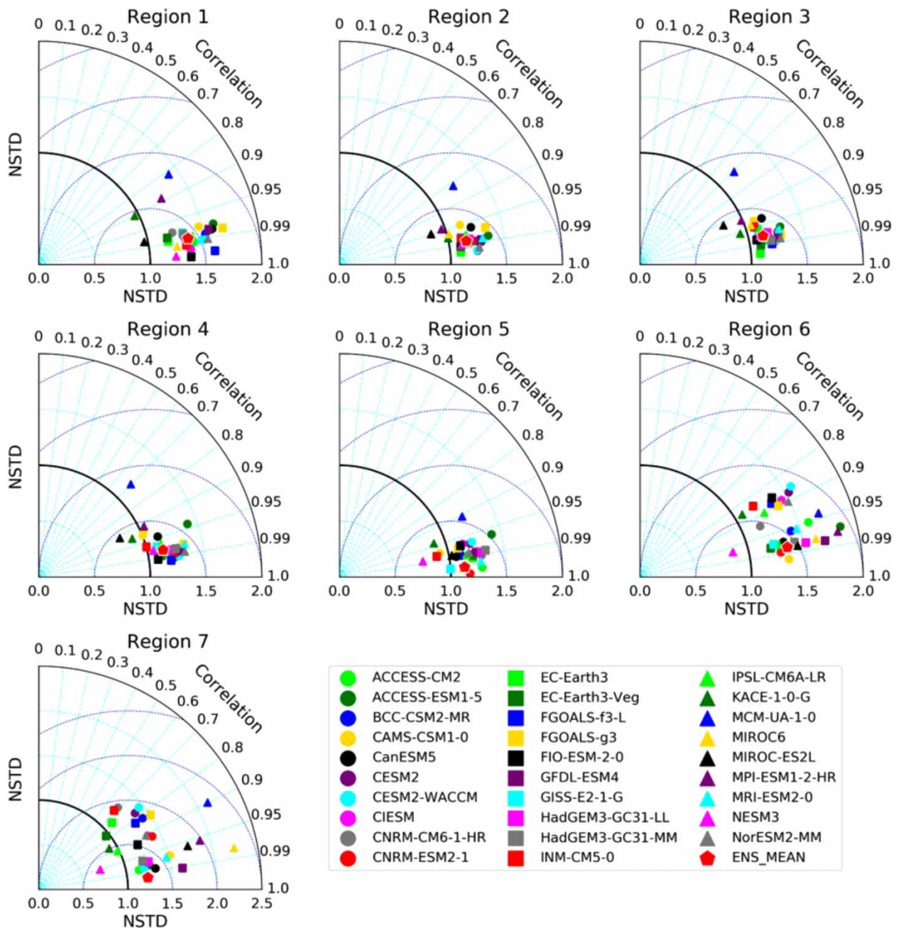
Figure 3 | Taylor diagrams of the GCMs' temperature annual cycles over the seven sub-regions of Vietnam.
