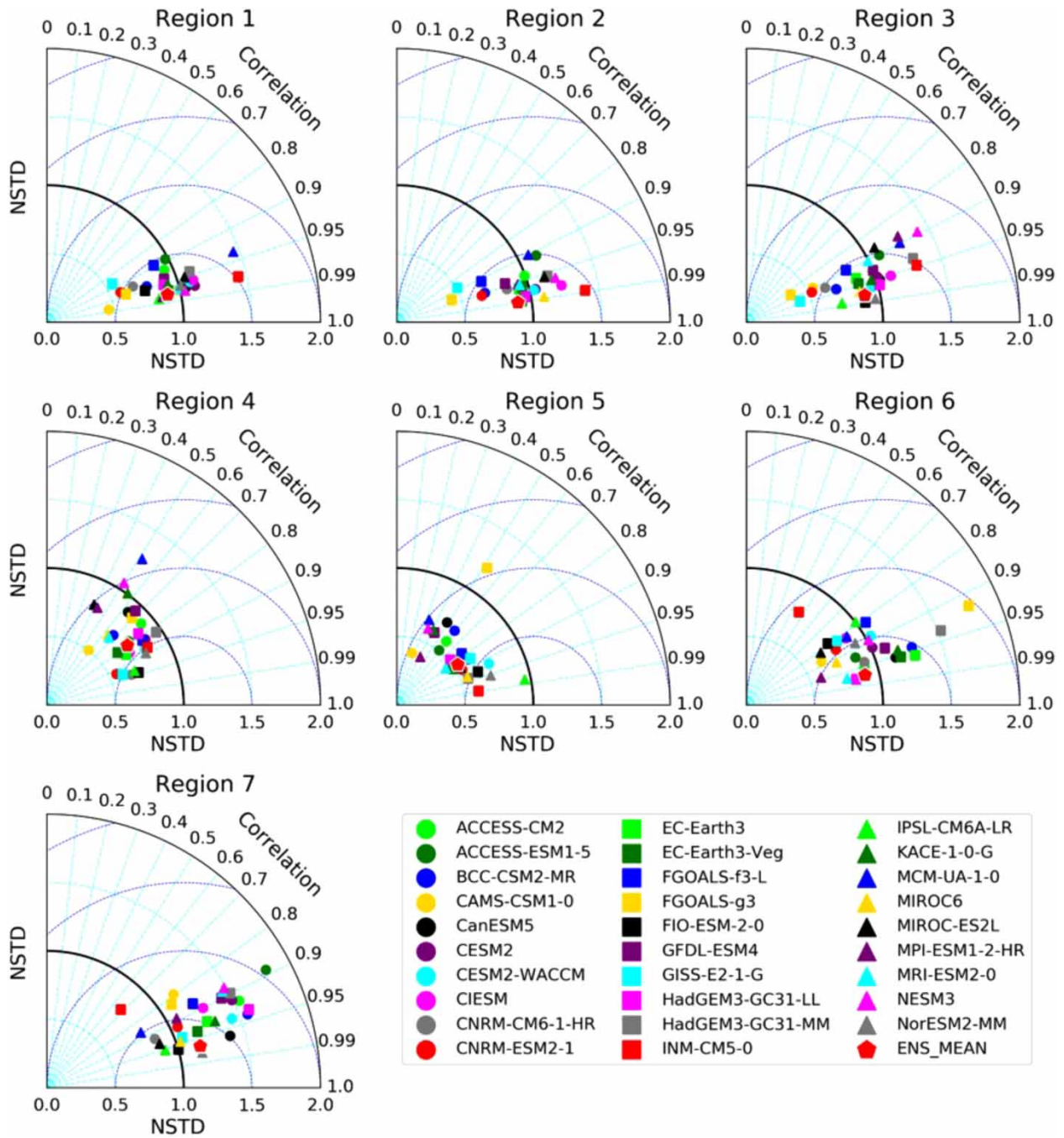
Figure 5 | Same as Figure 3 but for rainfall.
