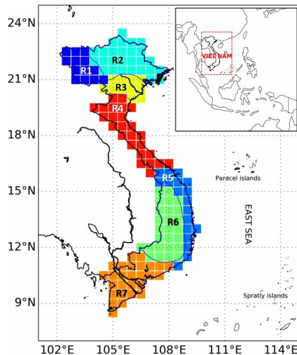
Figure 1 | Inland Vietnam and its seven climatic sub-regions. Grid cells with the size of 0.5^\circ \times 0.5^\circ are displayed. The inset map in the upper right shows the location of Vietnam within Southeast Asia.
