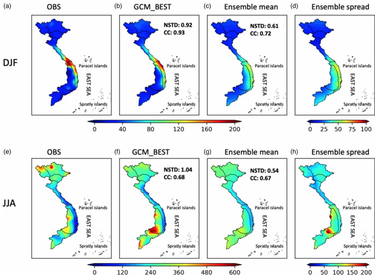
Figure 7 | Same as Figure 6 but for precipitation. Units in mm/month.
