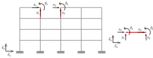
Fig. 6. Initial sub-structured problem with 6 degrees of freedom. On the left the NS, on the right the PS. The parts in red are exposed to ISO 834-1 fire curve. (For interpretation of the references to colour in this figure legend, the reader is referred to the web version of this article.)
