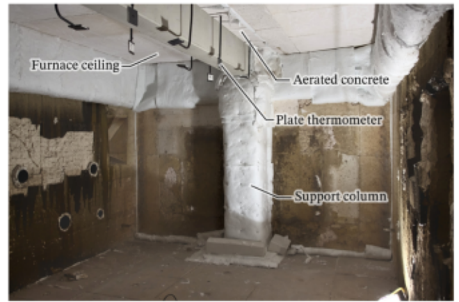
Fig. 11. Bottom view of the experimental setup.
