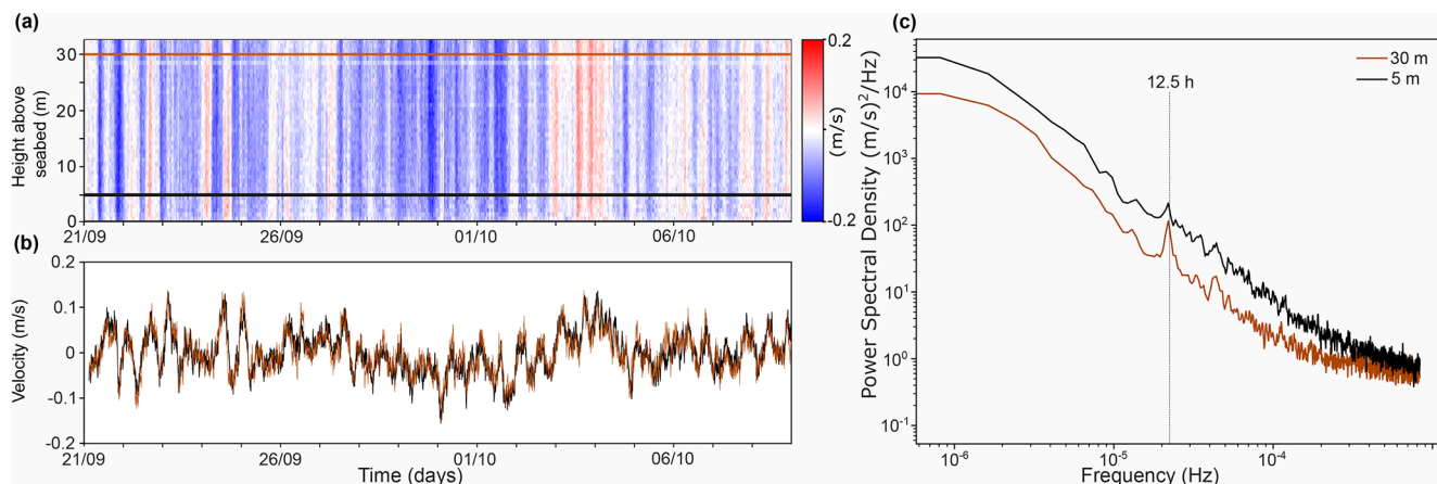
Figure 3. Velocity along the canyon ( V_{\text{along}} ) and frequency analysis at mooring M9 at 2170 m water depth for the period 21 September to 10 October 2019 when there was no turbidity current activity (see Fig. 2a for context). (a) Time series of V_{\text{along}} between 21 September and 10 October 2019. The horizontal brown and black lines indicate the heights above the seabed of the velocity time series displayed in (b) . (b) V_{\text{along}} speeds at 5 (black line) and 30 m (brown line) above the canyon floor. (c) Power spectral density computed for the whole time series (21 September 2019 to 15 January 2020) at 5 (black line) and 30 m (brown line) above the seafloor. Here, 12.5 h indicates the time period of the first frequency peak observed (frequency = 1/time).
