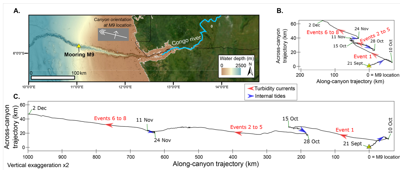
Figure 4. (a) Location of the moored ADCP (mooring M9) deployed in the Congo Canyon at 2190 m water depth. The aerial image of the Congo River mouth is taken from © Google Earth. (b) Hodograph showing residual currents measured at the mooring M9 location 30 m above the seabed. (c) Hodograph showing residual currents measured at mooring M9 location 5 m above the seabed. The start and end dates of turbidity current series recorded by the ADCP are marked. Red arrows show a downslope trajectory due to turbidity currents, whereas blue arrows show a net upslope trajectory due to internal tides.
