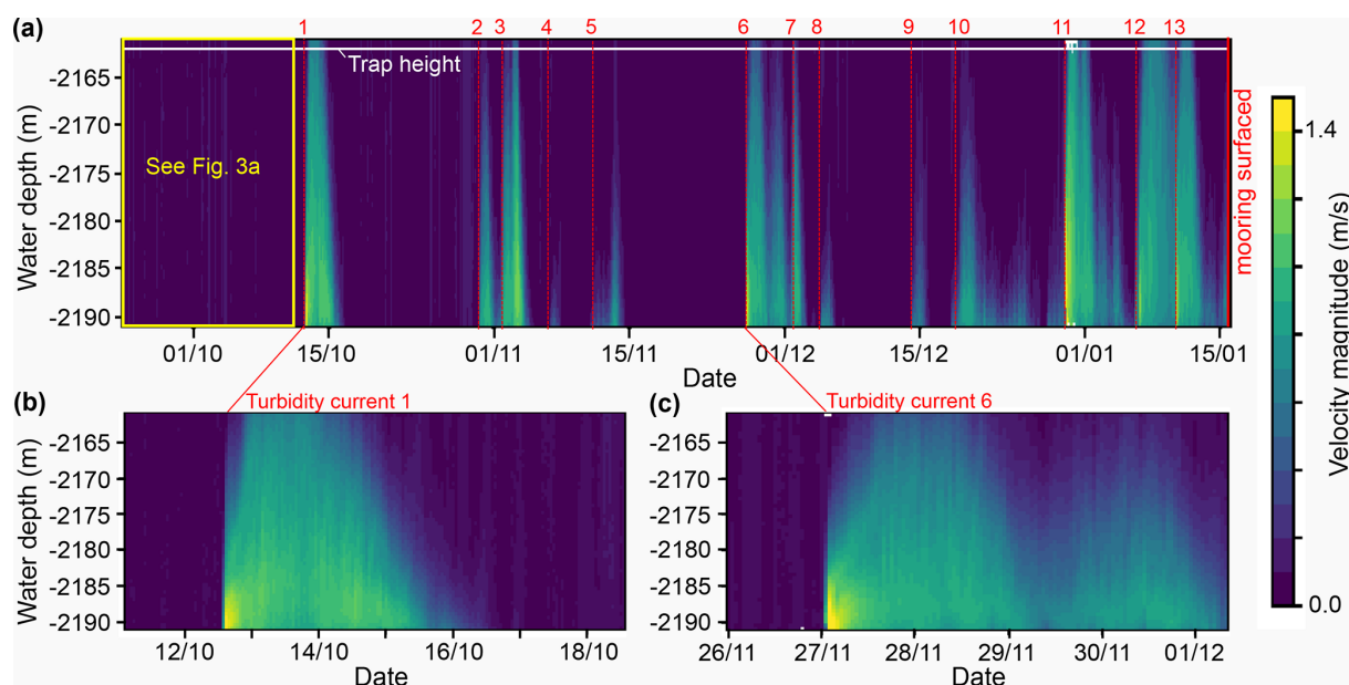
Figure 2. Velocity magnitude measured by a 600 kHz acoustic Doppler current profiler deployed 32 m above the seabed in the submarine Congo Canyon (see Fig. 1b for location). (a) Time series between 21 September 2019 and 15 January 2020. Numbers in red denote turbidity current events. (b) A zoomed-in view of turbidity current event 1. (c) A zoomed-in view of turbidity current event 6, which is made of two pulses.
