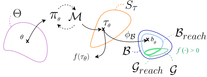
Figure 2: Notations overview. Each individual \theta \in \Theta define a policy \pi_\theta . This policy allows an agent to interact with an environment corresponding to a Markov Decision Process \mathcal{M} . The sequence of states and actions obtained after an evaluation on T steps is called the resulting trajectory \tau_\theta . This high dimensional vector is then projected in a behavior space \mathcal{B} through a behavior function \phi_{\mathcal{B}} , obtaining a behavior descriptor b_\theta in low dimensions. \tau_\theta also allow the computation of the fitness f(\tau_\theta) . The QD algorithm conducts its selection-mutation process using the resulting f(\tau_\theta) and b_\theta . The goal space \mathcal{G} is the subset of \mathcal{B} in which the corresponding trajectories have led to a non-null fitness.
