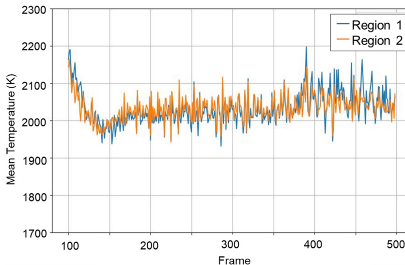
Figure 9. Mean temperature of ROIs 1 and 2 calculated for each frame of Experiment 1.
