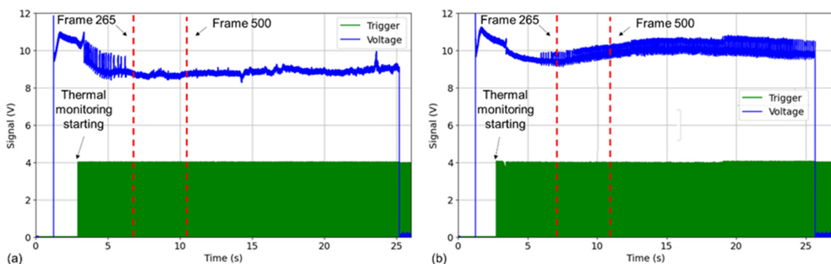
Figure 14. Voltage and trigger signals acquired for Experiment 3 (a) and 4 (b), as well as the positioning of captured frames.
