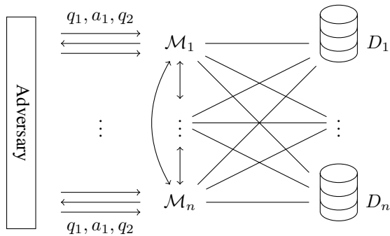
Fig. 1: Concurrent composition of interactive mechanisms, where the adversary can arbitrarily interleave its queries
