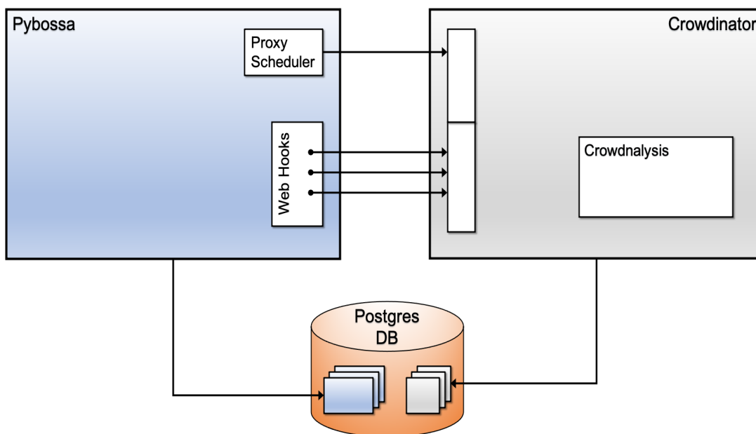
Figure 5.1.3. Providing Pybossa with intelligent scheduling.
