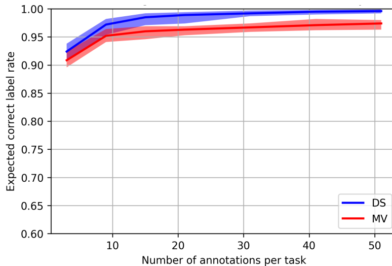
Figure 3.2.1.2. Prospective analysis for correct label rates for experts with Dawid-Skene Model (DS) and Majority Voting (MV) used for consensus.
