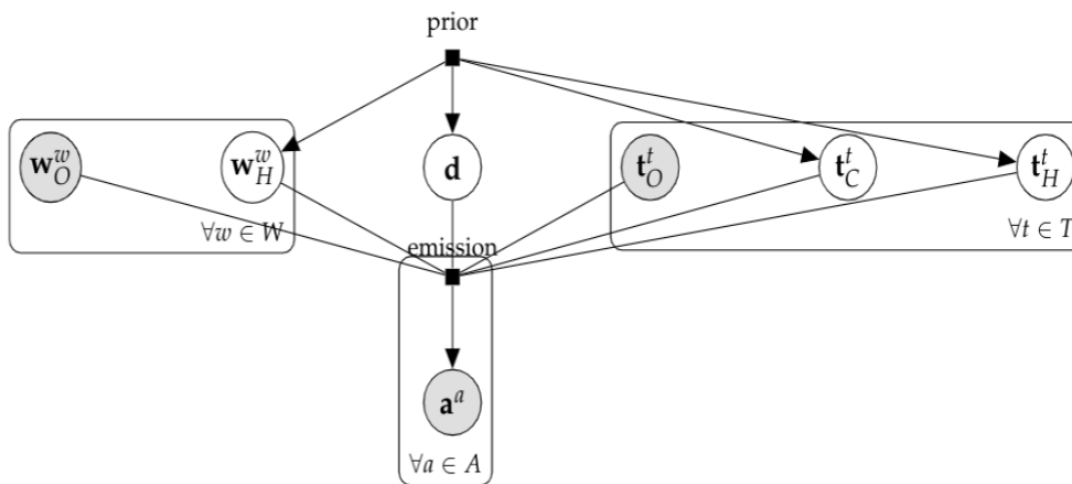
Figure 2.4.1.2. Probabilistic graphical model description of the abstract consensus model.
