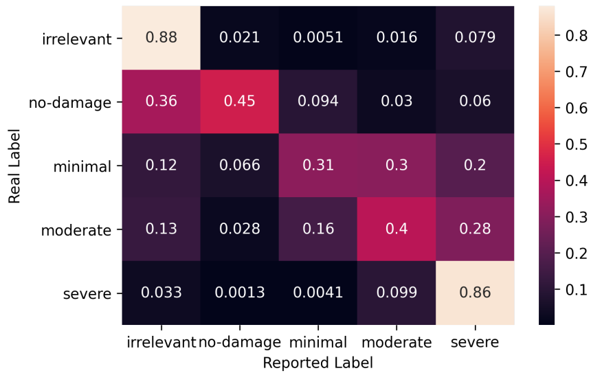
Figure 3.2.1.1. Error-rates of the experts in labelling the severity of damage.
