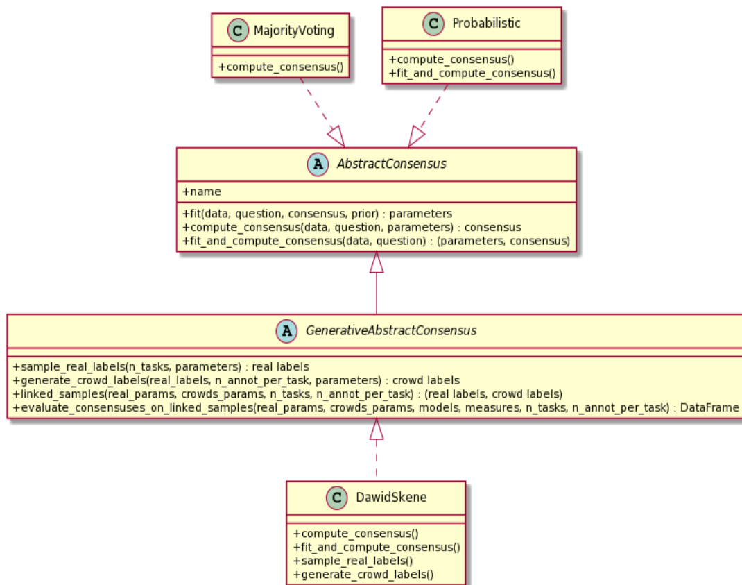
Figure 2.4.2.1. Class diagram of the Crowdanalysis library
