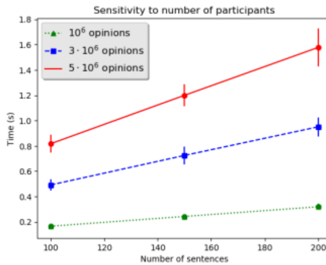
Figure 4.2. Computational time as the number of participants and arguments (sentences) grow.
