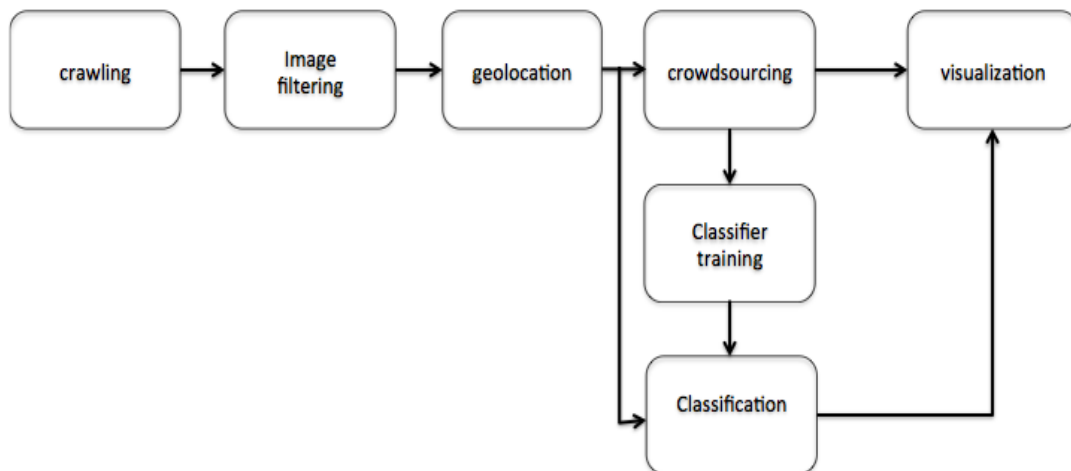
Fig. 8.1 - AI-enhanced pipeline
