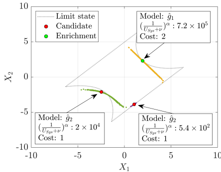
(b) Iteration 2
