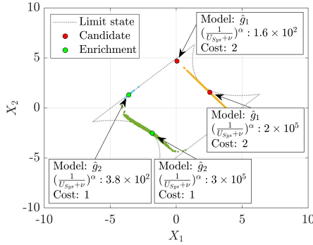
(a) Iteration 1
