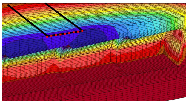
Figure 4 : Vertical displacement computed with ZSOIL. The nodes of interest are in red. A blue color corresponds to a 1.15cm settlement, and the red to 0cm
