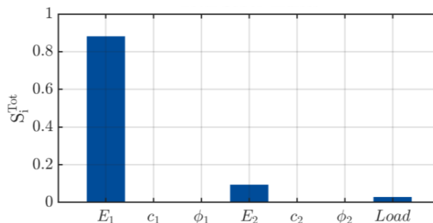
Figure 9 : Sobol total indices, which quantifies the influence of each input over the settlement
