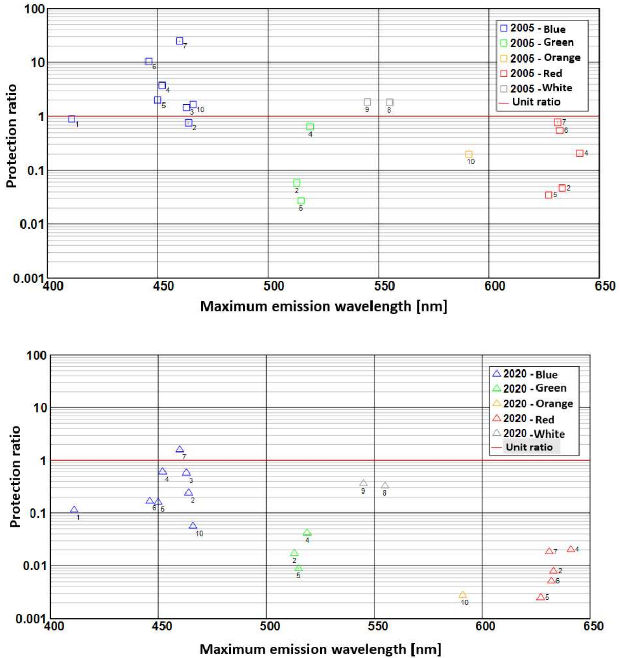
Figure 1: Ratios between the accessible radiation level and the limit value considered for the 19 LEDs contained in the 10 toys tested (2005 version of the standard above, 2020 below)
