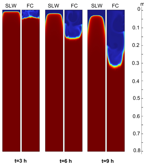
Figure 6. Contour of the ice volume fraction ( 1 - \theta ) for stagnant liquid water (SLW) and free convection (FC). A_p = 10 cm, H_{\text{dom}} = 0.8 m, and W = 1 m.
