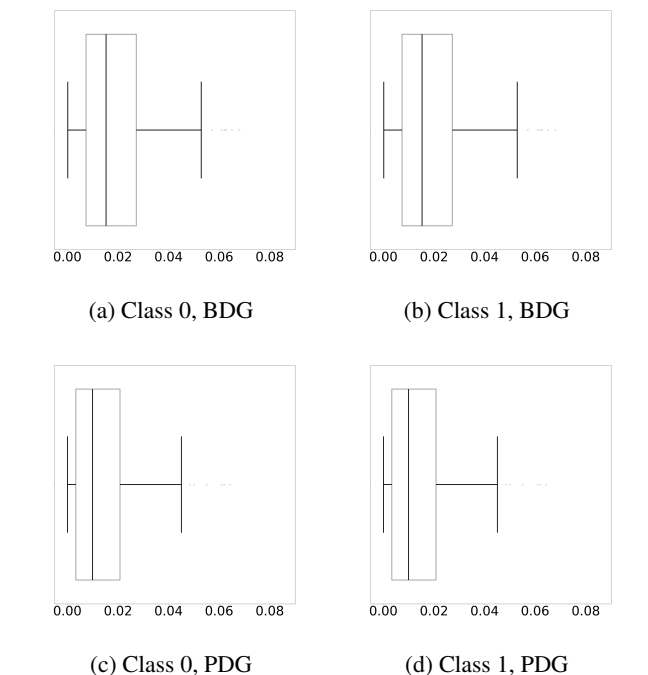
Figure 10: Box plots representing statistics of persistence of trust simplicial complex with \alpha = 0.98 for before and after data generation (vertically) and class 0 and class 1 (horizontally), respectively
