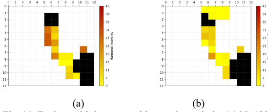
Fig. 11. Fault sensitivity maps with negative polarity (a) N=1200 inverters (b) N=228 inverters
