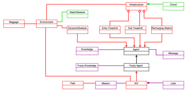
Figure 2. Simulator architecture: dynamic elements in red, static in green, and not related to the environment in purple.
