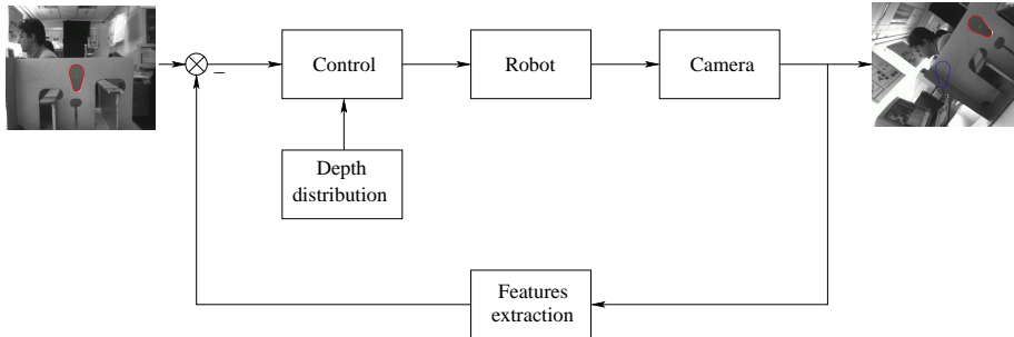
Figure 8: 2D visual servoing
