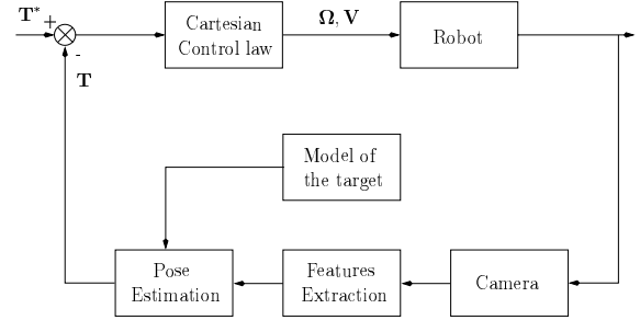
Figure 2: Block diagram of the 3D visual servoing
