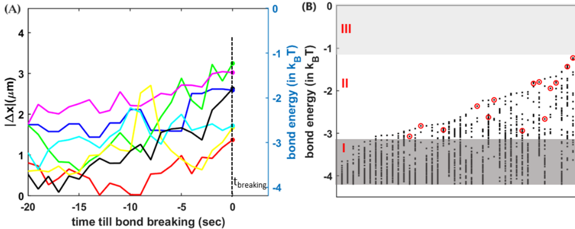
Figure 4: Bond breaking dynamics of flat-flat pairs: (A) Temporal evolution of |\Delta x| recorded from 20 seconds prior to breakage of the bond till the breaking time, t_{\text{breaking}} corresponding to 7 different flat-flat pairs formed at a depletant concentration of 0.01 mg/ml (left Y-axis) and the corresponding bond energies in units of k_B T (right Y-axis). The |\Delta x| at t_{\text{breaking}} is denoted by filled circles for each pair. (B) Bond energy values explored by various pairs of colloids in flat-flat configuration at 0.01 mg/ml depletant concentration. The bond energies at breaking is indicated by red open circles. Out of the 42 bonds represented here, 14 bond breaking events are observed.
