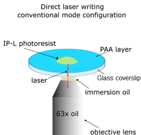
Figure S1: Schematic representation of the arrangement of the objective lens, the substrate and the resin droplet in conventional mode of direct laser writing
