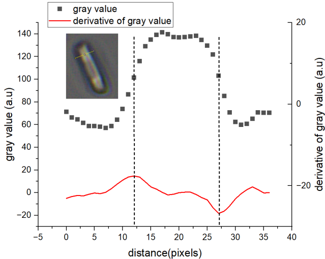
Figure S2: Gray scale profile (black dots) and its derivative along a line drawn across the width of a printed particle obtained from an optical microscopy image, with the particle lying on the substrate with its edge facing down. The image used for analysis is shown in the inset. The inflexion points, denoted by the maxima and minima of the derivative of gray scale profile represents the particle's edges. The distance between the two points gives the width of particle in pixels. In this picture, 20.8 pixels corresponds to 1\mu m .
