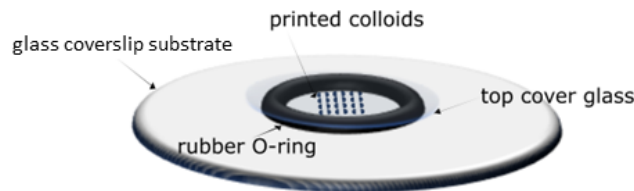
Figure S4: Schematics showing the experimental chamber used for observing the self-assembly of printed colloids. The schematic is not to scale: the glass cover slip is of 30mm diameter, the O-ring is roughly 5mm in diameter while the printed zone is typically of the order of 200\mu\text{m} \times 200\mu\text{m} .
