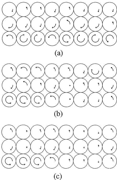
FIG. 7. Angular accelerations of particles at three stages of evolution of a rectangular array. The final stage is the steady state, where the accelerations do not evolve any more. The whole system has a translational acceleration of 0.1 g to the left with respect to the plane. The interparticle and particle-plane coefficients of friction are 0.1 and 0.2, respectively. The coefficient of friction with the walls is zero.
