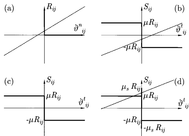
FIG. 3. (a) and (b). The equations of dynamics [cf. Eqs. (2.13) and (2.14)] projected on the local frame, attached to a contact between two particles, are shown as (dashed) straight lines with positive finite slopes. These cut Coulomb’s and Signorini’s graphs at a single point. (c) In static equilibrium, the slope is formally infinite (since \dot{\vartheta}_{ij}^t is kept zero) and the intersection with the two graphs is multiple valued. (d) When a friction law involving static and dynamic thresholds is considered, the solution is no more unique.
