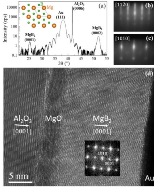
Fig. 1. (a) XRD spectrum measured on Al 2 O 3 /MgO(5)/MgB 2 (25)/Au(5) stack. In Inset is shown a scheme of two successive Mg and B planes along the MgB 2 [0001] growth direction, (b,c) RHEED patterns collected along two azimuthal directions ([1120] and [1010] MgB 2 respectively) separated by 30°. (d) HRTEM image captured along the \bar{1}\bar{2}\bar{1}0 zone axis of MgB 2 . Direct Fourier transform of MgB 2 TEM image is presented in inset.
