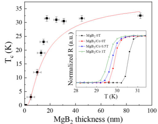
Fig. 2. MgB 2 critical temperature (black squares) as a function of the film thickness deduced from electrical resistance measurements as a function of temperature. The red curve corresponds to the theoretical variation based on the Cooper model taking account of the influence of an adjacent metallic layer on the T_c of a superconductor film. In inset are compared the R(T) for a single 25nm thick MgB 2 layer and a MgB 2 (25)/Co(5) bilayer under various applied in-plane magnetic fields.
