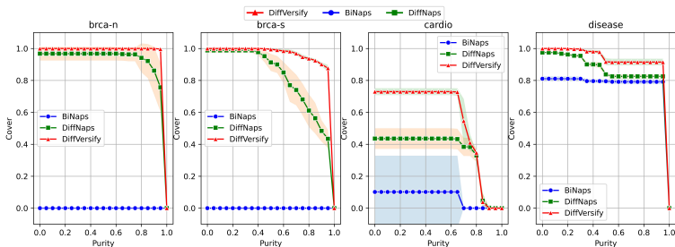
Fig. 1. ROC curve on four biology-related benchmarks, BRCA-N, BRCA-S, CARDIO and DISEASE over 5 runs.
