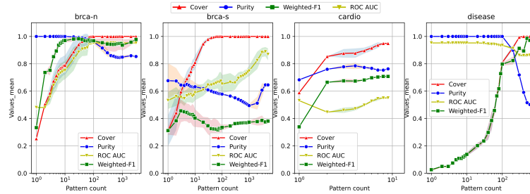
Fig. 2. Evolution of the performance metrics of DIFFVERSIFY over subsets of patterns defined by increasing COVER values across BRCA-N, BRCA-S, CARDIO and DISEASE over 5 runs.
