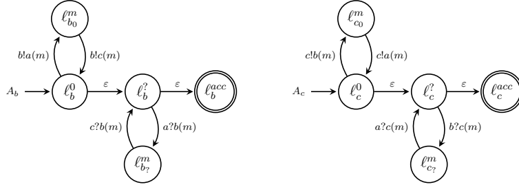
Figure 4: Sketch of A_b and A_c of \mathcal{S}_3 (only a single message m is considered).
