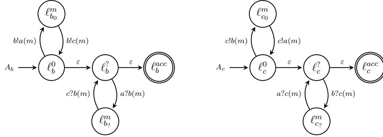
Figure 4: Sketch of A_b and A_c of \mathcal{S}_3 (only a single message m is considered).
