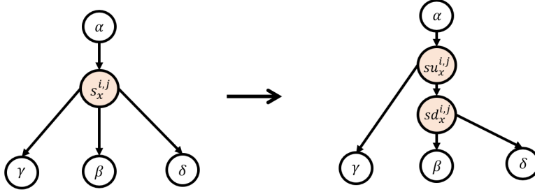
Figure 3: Transformation described by Lemma 3.4.
