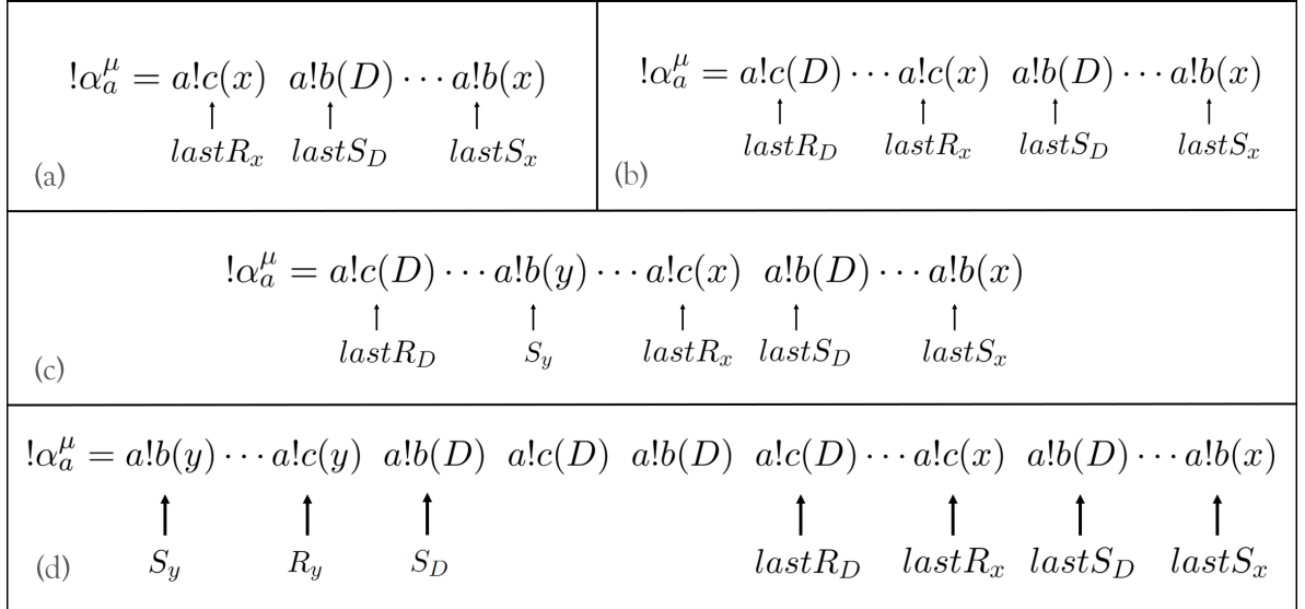
Figure 7: Examples of sequences of send actions executed by process a used in the proof of Lemma 4.12. Three dots between two actions indicate that there may be other actions in between.
