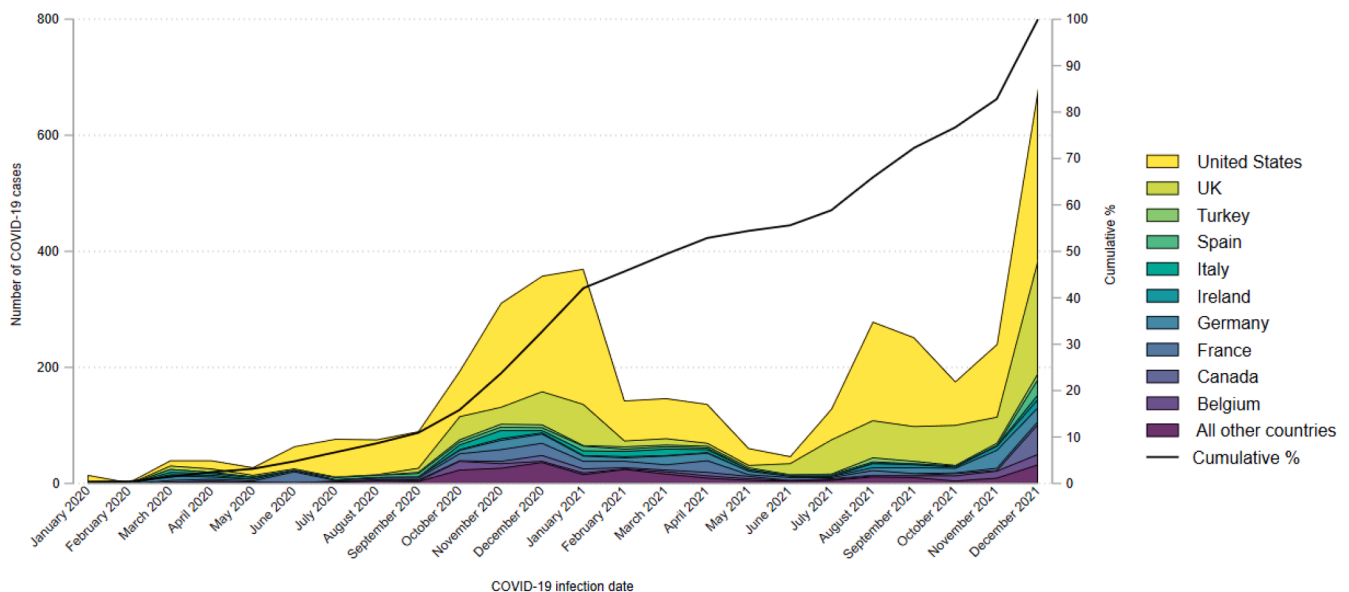
Fig. 2. The number of COVID-19 infections over time.
