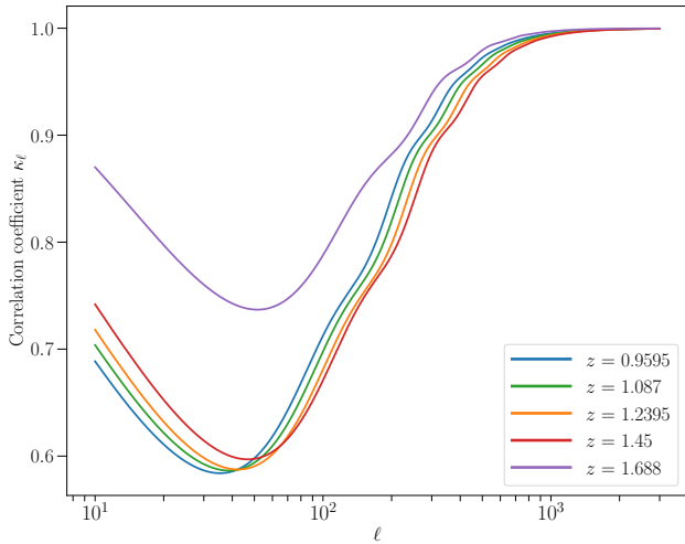
Fig. 5. Correlation coefficient \kappa_\ell between the two observables o_\ell and C_{\ell,sp} as a function of \ell .
