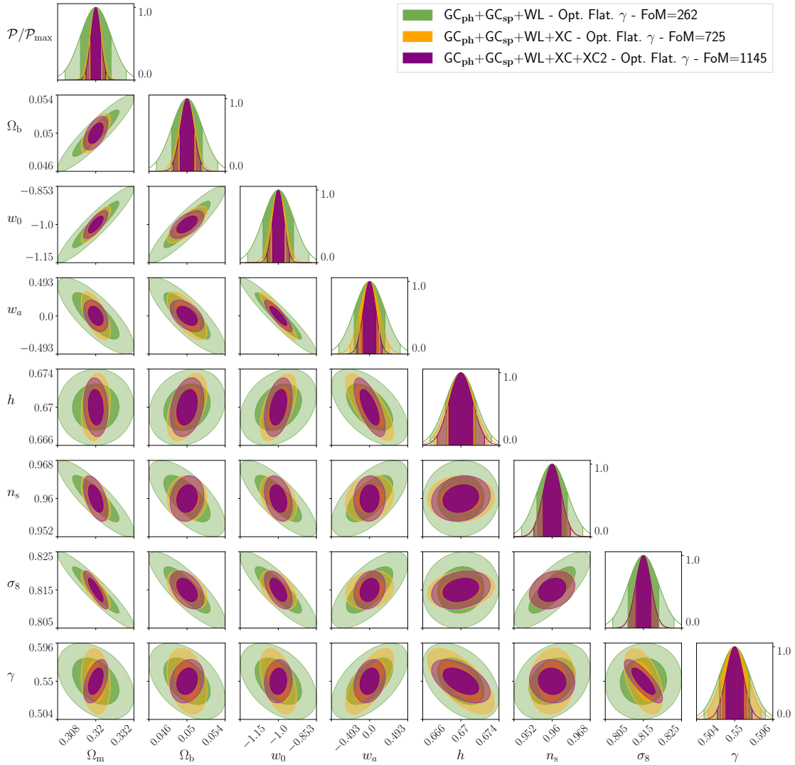
Fig. 3. 1D normalized likelihood ( \mathcal{P}/\mathcal{P}_{\max} ) and 2D marginalised Fisher constraints (with 1\sigma and 2\sigma limits highlighted) on cosmological parameters for different combinations of probes and in optimistic case/flat space with gravity model considered ( \gamma growth index parameter). The most stringent constraints are also obtained when including the new ratio observable (XC2).
