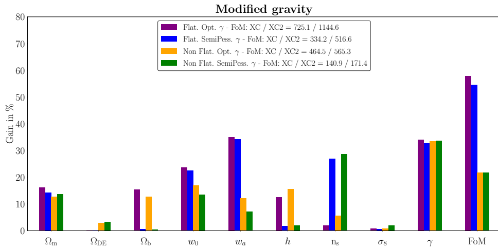
Fig. 4. Improvement on cosmological constraints from adding the new observable XC2 compared to the baseline analysis. The top panel shows the improvement for the semi-pessimistic and optimistic settings, and flat and non-flat cosmologies within general relativity. The bottom panel shows the equivalent figure for the modified gravity scenario including the growth index \gamma .
