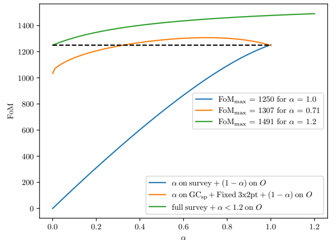
Fig. 6. Figure-of-Merit (FoM) as a function of the fraction \alpha of Euclid's observed sky ( f_{sky} ). The blue curve represents the combination of a fraction \alpha for the main probes (GC sp and 3×2pt) and (1 - \alpha) for the new observable O . The orange curve represents the combination of a fraction of \alpha for GC sp , together with the full 3×2pt analysis for the full survey and a contribution of (1 - \alpha) for the new observable O . The green curve shows the FoM of the full survey with an additional external contribution from the new observable up to a factor \alpha = 1.2 . The dashed line represents the optimal FoM using the standard GC sp and 3×2pt analysis. See the text for additional details on the different cases.
