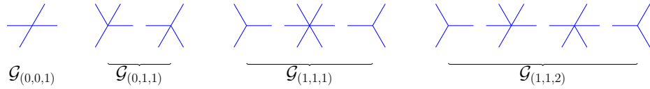
Fig. 6: Undecomposable Christoffel graphs.
