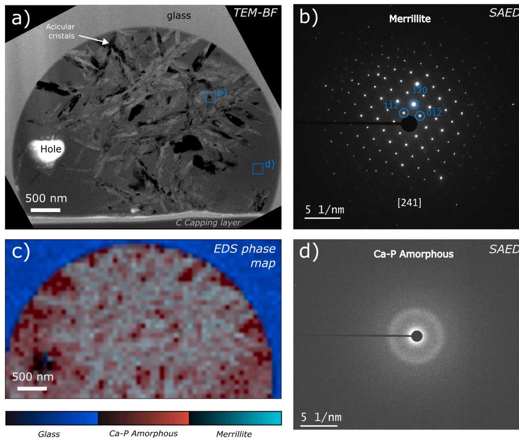
Fig. 5. TEM analyses of the phosphate-rich inclusion in the ICT. a) Bright field TEM image of the well-rounded inclusion. Acicular crystals are embedded in a smooth and homogeneous phase, i.e., amorphous P-rich glass. b) Selected area electron diffraction (SAED) pattern of the merrillite phase oriented along the [2,4,1] direction. c) Phase map based on the STEM-EDS spectrum image and obtained from linear mixing of reference spectra (Fig. S9). d) SAED pattern of the amorphous phase embedding the merrillite crystals.
