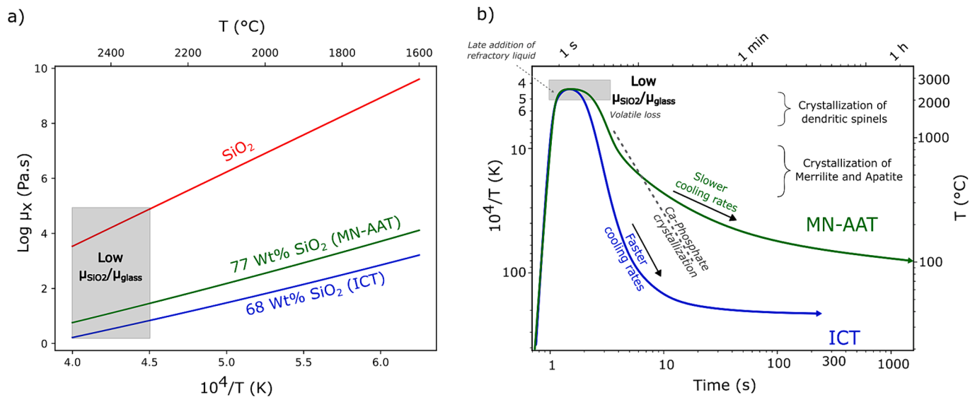
Fig. 13. a) Arrhenius plots for the viscosities of glass with various compositions. Viscosities are modeled using the three-parameter Tammann-Vogel-Fulcher (TVF) equation from (Richtet 1984; Toplis et al., 1997). The gray rectangle encloses the area where viscosity ratio; \lambda = \mu_{\text{SiO}_2} / \mu_{\text{glass}} is low. b) Schematic representation of the two thermal histories from ICT (blue) and MN-AAT (green) samples. Both samples are rapidly heated by the impact. MN-AAT reached a higher maximum temperature but for a short time before being ejected from the vapor plume and slowly cooled at the Earth's surface. ICT was heated to a lower temperature but remained in the plume longer, before being rapidly cooled in the atmosphere. Fe-rich glass in MN-AAT originates from a late addition of material in the glass.
