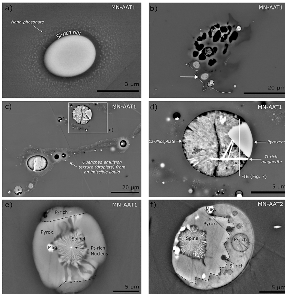
Fig. 3. Back-scattered electron images of phosphate-rich inclusions in MN-AAT (see also Fig. S5). a) A single-phase phosphate-rich inclusion in the MN-AAT section. Most inclusions appear homogeneous and single-phased. A ring of Si-rich glass surrounds the inclusion. Ca-phosphate nano-spheres also mantle the inclusion. The larger spheres are closer to the inclusion. b) Multi-phase inclusions embedded in lechatelierite (white arrow). Lechatelierite frothy texture is due to the high density of vesicles resulting from decompression. c) Complex multi-phase inclusions embedded in a SiO 2 -rich flow band mixed with phosphate nanospheres. d) BSE image of a representative inclusion in MN-AAT (Fig. S6). Several phases are visible. The change in volume due to the crystallization of the minerals is marked by dark and empty areas. Localization of the FIB section is indicated. e-f) Recurrent mineral assemblage observed in phosphate-rich inclusion (Fig. S7). A Pt-Ru-rich nucleus facilitated the crystallization of a spinel which is enclosed by a pyroxene and a phosphate phase (Fig. S8). P-rich = Phosphate riche phase, Pyrox. = pyroxene, Mag. = Magnetite.
