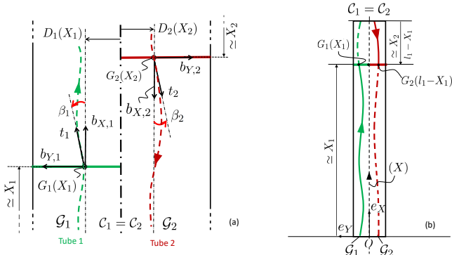
Figure 5. (a) : Lateral view of a piece of a 2-tube planar CPPR at rest, with non-parallel curved centroid lines. Referring to Section 2.5, \beta_i is a design shearing parameter measuring the angle between b_{iX} and t_i = (dr_i/dX_i) (see also Extension 2). (b) : Geometry of the same CPPR in its resting configuration with curved centroid lines, in the baseplate frame (O, e_X, e_Y, e_Z) . X_1 and X_2 are the arc lengths of the continuous green and red lines, counted from the base and tip of the CPPR respectively, with their "straight" approximations on both sides as in Remark 4.
