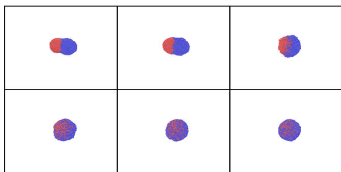
Figure 11. Snapshots obtained in the heating of Janus AuNi nanoparticles (6125 atoms, where 3061 atom of Au and 3064 of Ni) with heating shown in Figure 3S. T_{\max}=2700\text{K} , time delays are 0, 10, 20ps (upper row) , 50, 70, and 90 ps (bottom row), from left to right.
