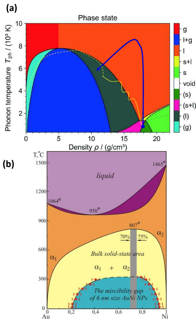
Figure 2. (a) - Temperature-density phase diagram of gold with phase states (61): s—solid; l—liquid; g—gas; l + g—liquid-gas mixture; s + l—melting; (s)—metastable solid; (s + l)—metastable melting; (l)—metastable liquid; (g)—metastable gas. bn and sp are binodal and spinodal curves, respectively. (b) - Binary Au-Ni phase diagram (63,64,65).
