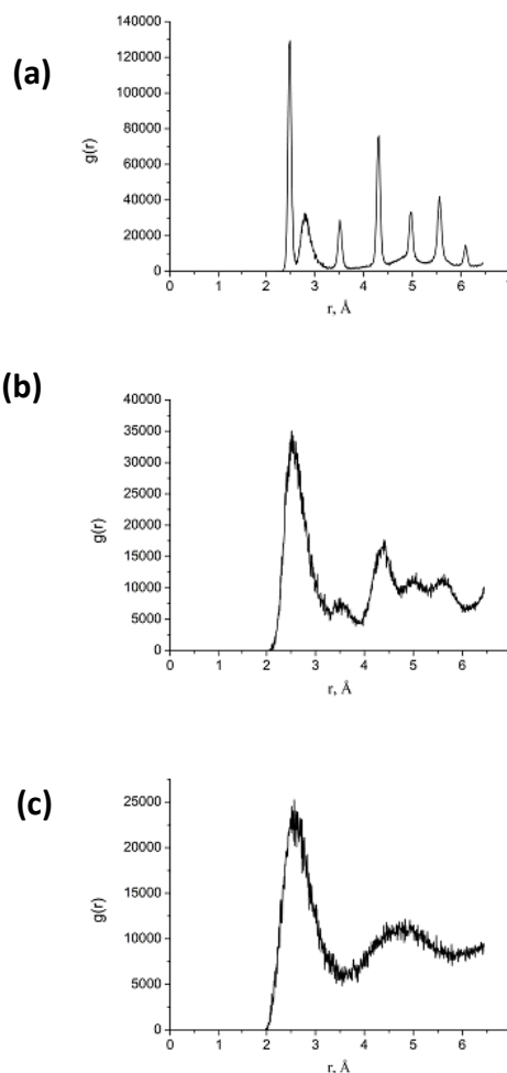
Figure 12. RDF calculated for the AuNi Janus nanoparticle shown in Figure 11 at time delays (a) 0ps, (b) 10ps, and (c) 20 ps. Here, the maximum temperature T_{\max}=2700\text{K} .
