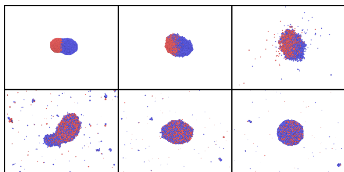
Figure 14. Simulation snapshots for AuNi Janus NP and T_{\max}=8000\text{K} , at time t=10, 20, 30, 50, 70, 90 ps.
