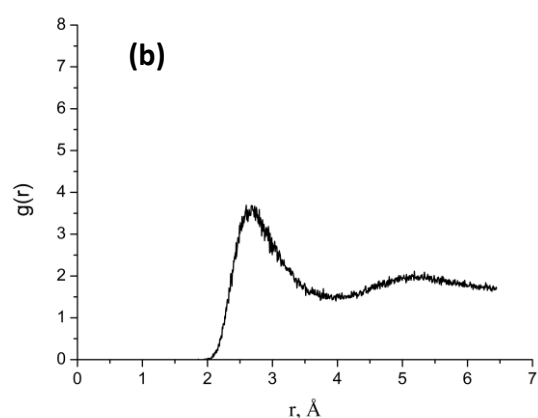
Figure 15. Calculated radial distribution function (RDF) for Au cluster with R=20\sigma_c , (a) – at t=0.1 ps and (b) – at t=10 ps. In figure (a) all the results correspond to Au cluster with R=50\sigma_c showing partial melting that is then completed in (b). Calculated radial distribution function (RDF) (50) for Au cluster with radius R=50\sigma_c obtained at t=10 ps.
