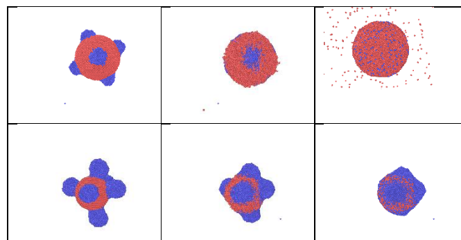
Figure 15. Simulation snapshots for AuNi core-satellite NP and time delay of 0, 15, and 160 ps ( 6500\text{K} ), where gold nanoparticle R=40 uc, and Ni R=10 uc, symmetric Ni NP's distribution, and for T=3500\text{K} where gold nanoparticle R=40 uc, and Ni R=14 uc ( 1 uc = 0.352 nm for Ni), non-symmetric Ni NP's distribution.
