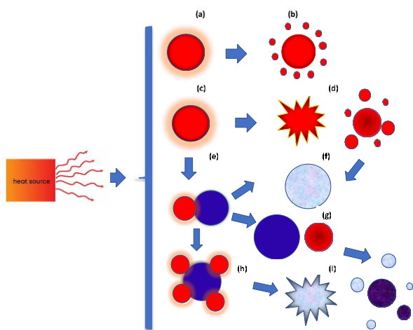
Figure 3. Schematics of nanoparticle transformations under fast heating: (a)-(b) -evaporation, (c)-(d) -fragmentation, (d)-(e) sintering, (e)-(f) and (d)-(f) -alloying, (e)-(h) aggregation, (h)-(i) -fragmentation of an aggregate.
