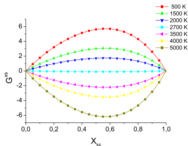
Figure 10. Excess energy, as depicted in Fig. X, is calculated using the following equation for AuNi alloy (63-65), eq. (S1). Energy units are J/K mol.
