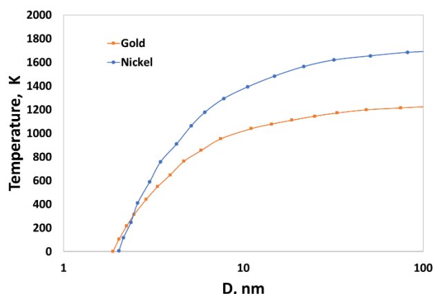
Figure 1. Size-dependent melting temperature of gold and nickel nanoparticles (59-60).
