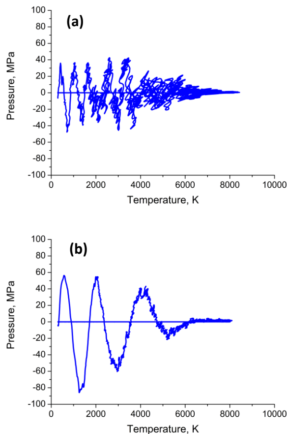
Figure 8. Calculated pressure-temperature dependencies (a) for Au nanoparticle with radius R=20 uc ; (b) - the same for radius R=50 uc. The heating-cooling conditions are the same as in Fig. 4-7.
