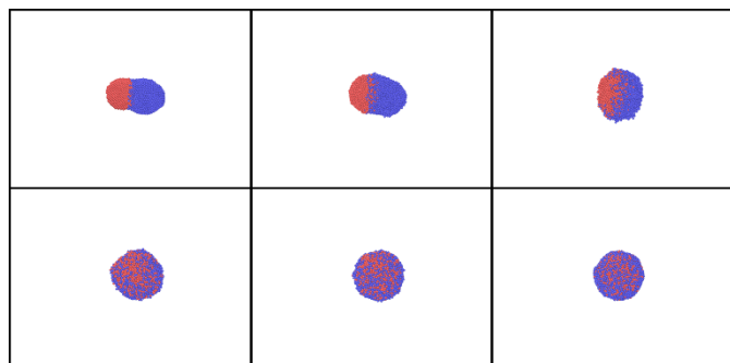
Figure 13. Simulation snapshots for AuNi obtained at time delays t=0, 10, 20, 50, 70 and 90 ps for T_{\max}=4000\text{K} .
