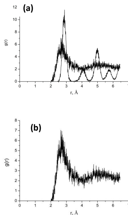
Figure 6. Calculated radial distribution function (RDF) for Au cluster with R=20 uc, (a) at t=0.1 ps and (b) -the same at t=10 ps.
