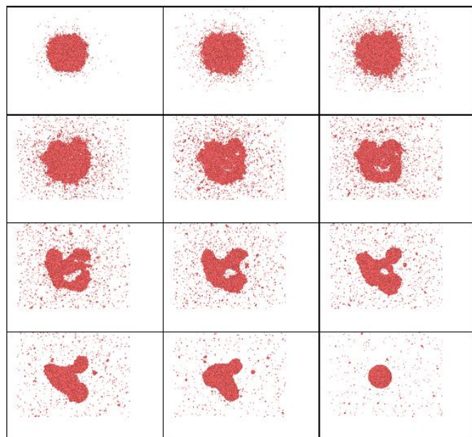
Figure 5. Snapshots obtained in MD simulations showing the time evolution of Au nanocluster with radius R=50 uc (uc is unit cells length, 0.407 nm for Au), N=30845 atoms and maximum temperature T_{\max}=8000\text{K} obtained at time delays t=0.1, 5, 10 ps (first row), 20, 30, 40ps, (second row), 50, 60, 70ps (third row), 80, 100, 150 ps (bottom row) after the beginning of strong and short (20ps) heating (from left to right).
