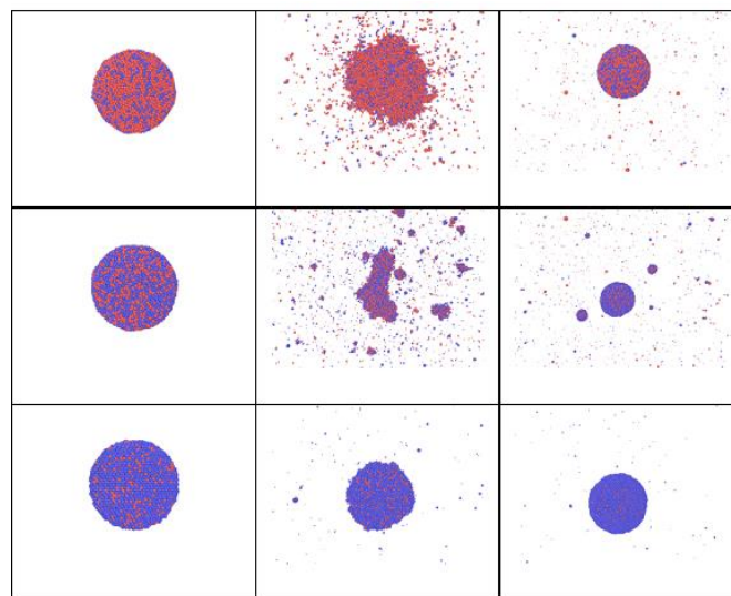
Figure 9. Snapshots obtained in MD simulations for AuNi nanoparticle ( R \sim 40 uc, N \sim 15820 atoms) heated up to 9000K and cooled down to 300K, showing the role of composition for time delays of 0, 50, and 160 ps for three Ni fractions (top - 20%, middle row - 50%, bottom - 80%).
