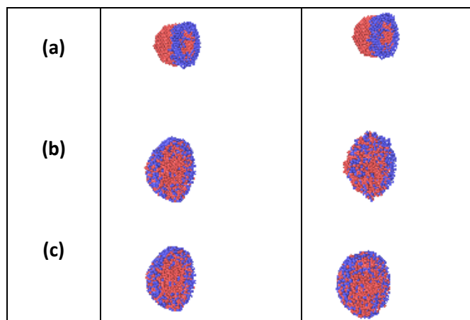
Figure 25. Snapshots obtained in the heating of Janus AuNi nanoparticles with heating shown above. Slice view calculated at 5, 80, and 100 ps, the left column is for T_{\max}=400 and the right one is for T_{\max}=2700 K.
