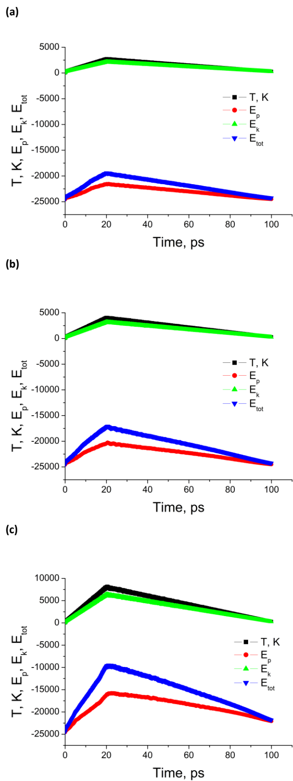
Figure 3S. Calculated temperature and NP energies vs time for AuNi Janus NP and T_{\max} = 2700\text{K} (a), 4000\text{K} (b), and 8000\text{K} (c). Energy units are cal/mol.
