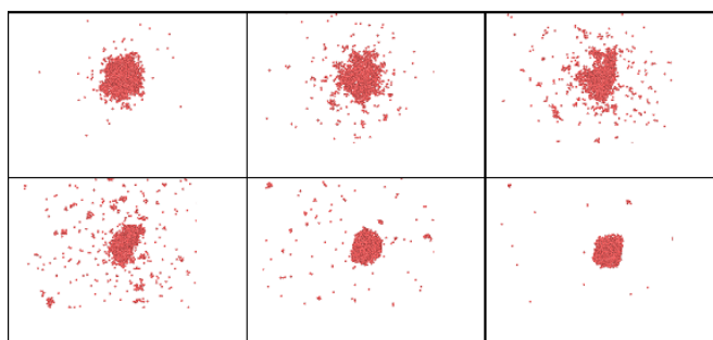
Figure 4. Snapshots from MD simulations showing the time evolution of Au nanocluster with radius R=20 uc ( 1\text{uc} = 4.07 \text{ \AA} for Au), N=1959 atoms, and maximum temperature T_{max} = 8000 K obtained at t=0.1, 5, 10 ps (upper row), 20, 50, 100 ps (bottom row) from left to right.
