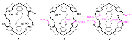
Scheme 1. Chemical structures of compounds 1-3 . Only a single enantiomer
