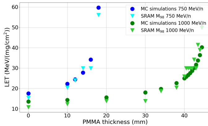
Fig. 6. Comparison between LETs estimated with FLUKA MC and those determined from the SRAM MCUs with the M98 parameter for different ion beam primary energies and at varying thickness of PMMA degrader.
