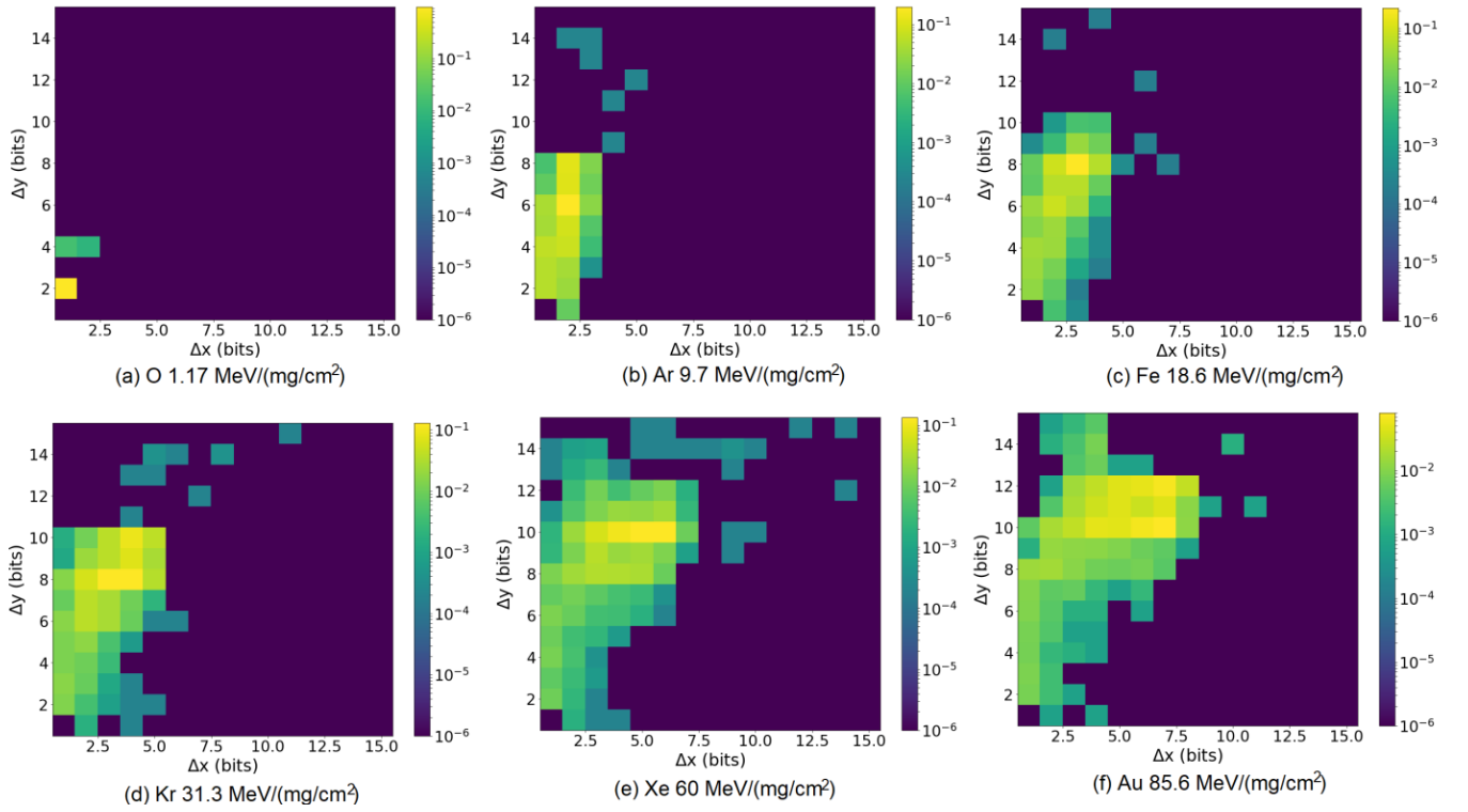
Fig. 8. Heatmaps of MCU clusters based on the combinations of \Delta x - \Delta y for the data collected at RADEF.
