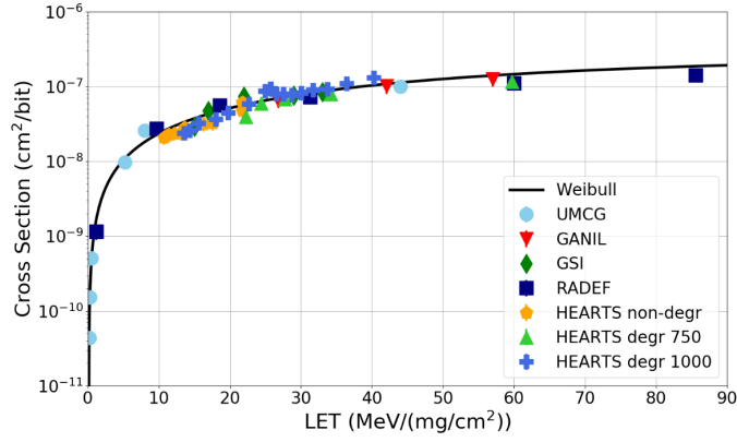
Fig. 1. SEU cross section as a function of LET for this memory measured at the five facilities.
