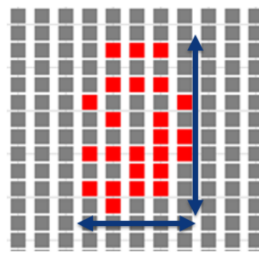
Fig. 7. Example of a cluster with multiplicity of 24 with indication of the \delta x and \delta y dimensions.
