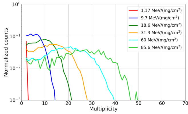
Fig. 4. Histogram of ion multiplicity for the MCUs collected with the beams at RADEF.
