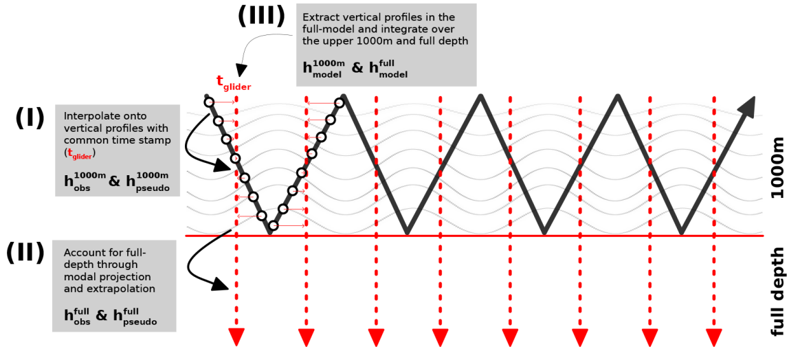
Figure 6. Schematic illustrating (I) the linear interpolation of vertical displacements for a given profile onto a common time stamp t_{glider} prior to the vertical integration to obtain h_{obs}^{1000m} and h_{pseudo}^{1000m} , (II) the modal projection on climatological modes and extrapolation to the full-depth range to obtain h_{obs}^{full} and h_{pseudo}^{full} , and (III) the vertical extraction in the full model at t_{glider} to obtain h_{model}^{1000m} and h_{model}^{full} .
