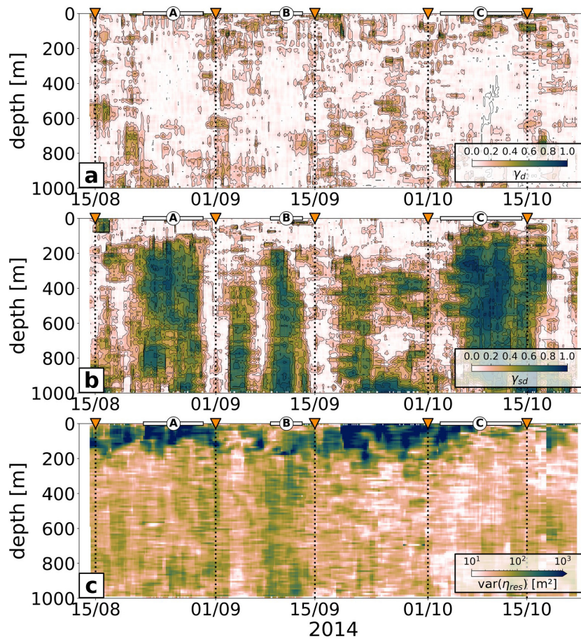
Figure 7. Explained variance by the (a) diurnal ( \gamma_d = cov(\eta_d, \eta)/var(\eta) ) and (b) semidiurnal ( \gamma_{sd} = cov(\eta_{sd}, \eta)/var(\eta) ) internal tide as given by the sinusoidal fit applied on the glider observations. (c) Variance of the residual signal var(\eta_{res}) .
