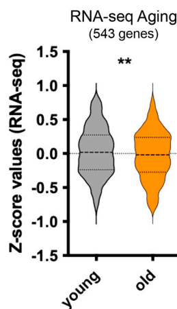
Fig. 4. Neuronal enhancers are regulated in an opposite way in aging and advanced tauopathy. (A) Gene Ontology analysis of the selection of neuronal enhancers (543 genes; Supplementary Fig. 7) using GREAT showing Cellular Component and Biological Process. (B,C) SeqMINER metaprofiles performed on these neuronal enhancers in the different contexts: old versus young mice presented H3K27ac-depleted levels in the gene body of these genes, while 12-month-old Thy-Tau22 mice displayed an enrichment of H3K27ac levels compared to the WT mice. (D,E) Z-score values of the neuronal genes expression, obtained from the RNA-seq data, showing a significant decrease of their expression levels in the aging mouse model and a significant increase in the tauopathy mouse model. Student t-test, Bonferroni correction test ** p < 0.01 ; **** p < 0.0001 .
