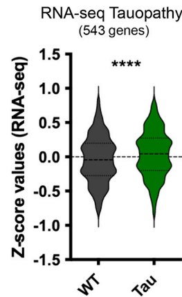
Fig. 4. Neuronal enhancers are regulated in an opposite way in aging and advanced tauopathy. (A) Gene Ontology analysis of the selection of neuronal enhancers (543 genes; Supplementary Fig. 7) using GREAT showing Cellular Component and Biological Process. (B,C) SeqMINER metaprofiles performed on these neuronal enhancers in the different contexts: old versus young mice presented H3K27ac-depleted levels in the gene body of these genes, while 12-month-old Thy-Tau22 mice displayed an enrichment of H3K27ac levels compared to the WT mice. (D,E) Z-score values of the neuronal genes expression, obtained from the RNA-seq data, showing a significant decrease of their expression levels in the aging mouse model and a significant increase in the tauopathy mouse model. Student t-test, Bonferroni correction test ** p < 0.01 ; **** p < 0.0001 .
