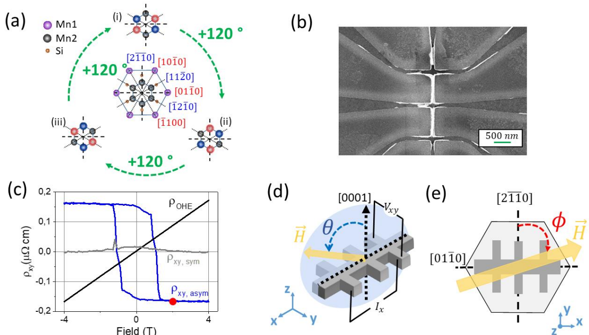
Figure 1. (Color Online) (a) Representation of the hexagonal unit cell of the altermagnetic phase of Mn 5 Si 3 , consisting of two magnetically ordered opposite-spin sublattices of Mn2-atoms, highlighted in red and blue. The 3 possible variants rotated by 120° are shown. (b) Scanning electron microscopy image of the ~100 nm-wide Hall cross structure used in this work. The white highlighted foil is mostly the negative resist MaN2403, which was burned during ion etching. Re-deposition only around the corners of the Hall bar's arms cannot be excluded, due to the small size of the device. See also Fig. S5. (c) The 3 contributions to the field ( H )-dependence of the transverse resistivity, \rho_{xy} , measured at T = 110 K, for H along [0001] . (d,e) Representations of the experimental design, highlighting the \theta polar angle used for field-sweep on a given plane. Plane change was achieved by varying the \phi azimuthal angle.
