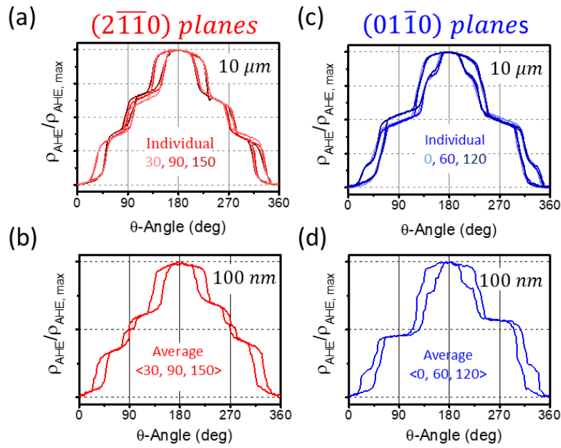
Figure 4. (Color Online) (a,c) Superposition of the individual Hall signals, when \mathbf{H} is rotated in the (2\bar{1}\bar{1}0) plane and its two equivalents [(0\bar{1}\bar{1}0) , respectively], measured for a 10 \mu\text{m} -wide Hall bar containing all three variants [Figure 1(a)]. (b,d) Averaged Hall response over all signals obtained in Figure 2(b,d,f) [(a,c,e), respectively], when \mathbf{H} is rotated in the (2\bar{1}\bar{1}0) plane and equivalents [(0\bar{1}\bar{1}0) , respectively], i.e. for \phi = 0, 60, 120^\circ ( \phi = 30, 90, 150^\circ , respectively), for a 100 \text{ nm} -wide Hall cross containing mainly one altermagnetic variant (see Figure 2 for the individual signals).
