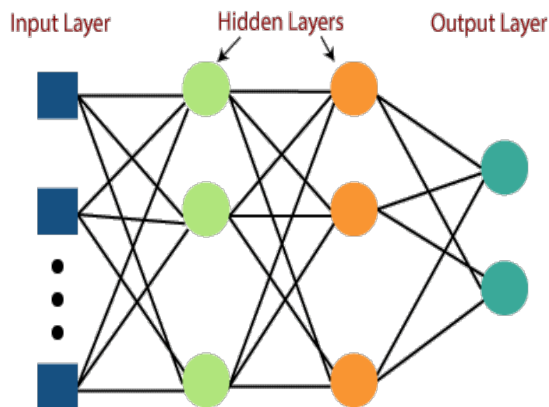
FIGURE 3.2.1 – MLP Architecture. [100]
