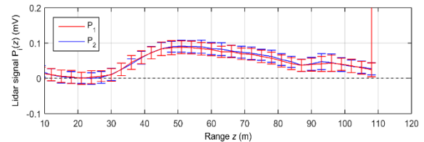
Figure 3: OSAS-Lidar signal for the active channel (red) and the reference channel (blue). The background noise signal is numerically subtracted. Each signal corresponds to a 1 second average time.
