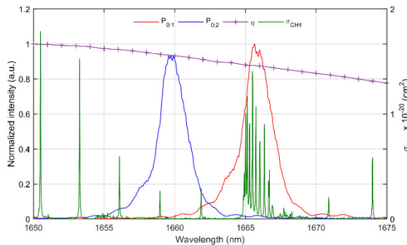
Figure 1: OSAS-principle applied to the 2\nu_3 Methane gas absorption band. The PSD of a broadband light source is spectrally shaped matching (red curve) or not (blue curve) the absorption cross-section spectrum \sigma_{CH_4}(\lambda) (green lines) In purple, the opto-electronic efficiency spectrum \eta(\lambda) of the OSAS detection part.
