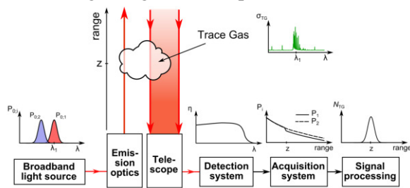
Figure 2: Principle of OSAS-lidar. Two different laser pulses are alternatively generated. Using a lidar system, these two emitted laser pulses through the atmosphere undergo different absorptions due to the TG presence, giving rise to the output OSAS-lidar signals S_1(z) and S_2(z) , after collection by a lidar receiver and detection on a photoreceptor.
