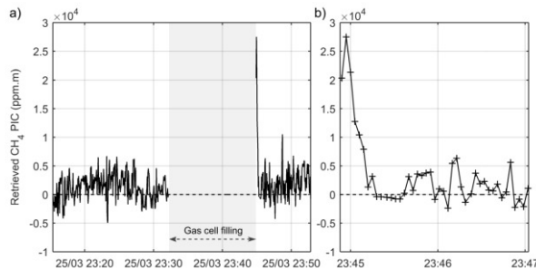
Figure 4: a) Retrieval of methane path integrated concentrations. The gas cell was closed during methane filling. b) Methane concentration dispersion. Once the gas cell opened, the methane concentration decreases quickly to the detection limit in less than 30 seconds.
