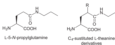
Figure 4. New derivatives of \text{L-theanine} : potential NMDA receptors agonist or co-agonist.
