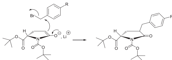
Scheme 2. Stereospecific alkylation of the lithium enolate of ( S )- N -Boc-Pyr-OrBu, 1 .
