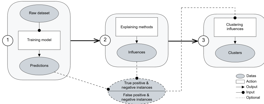
Figure 2: Our proposed Framework for explanation analysis.
